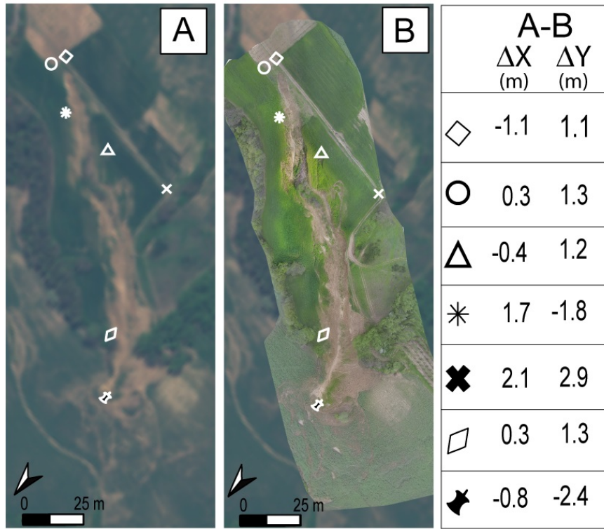
Fig. 2. Figure 3. Position of the seven GCPs used to evaluate the co-registration of WordView-2 satellite image (A) and UAV image (B). Corresponding points are illustrated with the same symbol. Differences of
