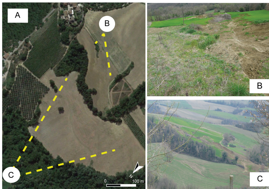
Fig. 3. Figure 4. (A) Overview of the Assignano landslide area in Google Earth™ taken on 8 July 2013. Photo shooting points and photograph taken (B) close to the landslide and (C) from a viewpoint. The photog
