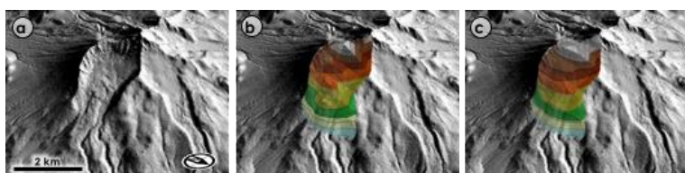
Figure 12: Bird-eye views of the reconstructed source area of the sector collapse. (a) Present topography of the scar. (b) 3D TIN of reconstructed surface of the original mountain body by linear extrapolations. (c) 3D TIN of reconstructed surface of the original mountain body by Bézier curve fitting.
