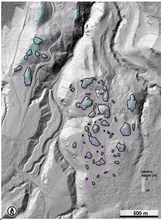
Figure 6: Map of the hummocks extracted in the study area (n = 65). Blue to purple colors show the sink-filled areas on the inverse DEM, indicating the locations of local mounds and ridges. Black solid lines represent the mound boundaries of hummocks identified. Note that not all the sink-filled areas are identified as hummocks, based on the interpretation of orthorectified images and field observations. Hillshade images are derived from RPAS-derived 36-cm DEM (foreground) and 10-m PRISM-DEM (background).
