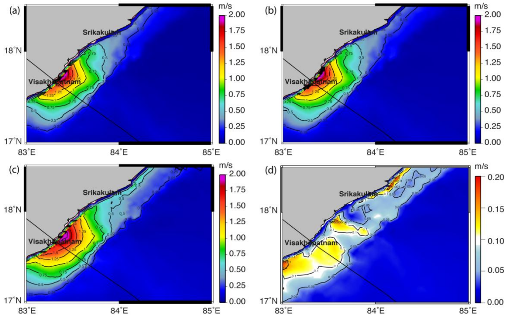
Fig. 5. Spatial distribution of maximum surface currents (m/s) due to (a) winds, (b) winds and tides and (c) winds, tides and waves, during cyclone, (d) difference in current speeds from (b) and (c), illustrating change in current speeds due to wave-current interaction (colour code represents current speeds in m/s).
