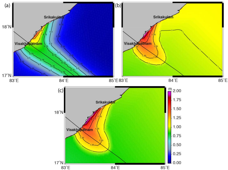
520 Fig. 3. Spatial distribution of maximum surface elevation (m) due to (a) cyclonic winds, (b) cyclonic winds and tides and (c) cyclonic winds, tides and waves (colour code represents surface elevation in m).
