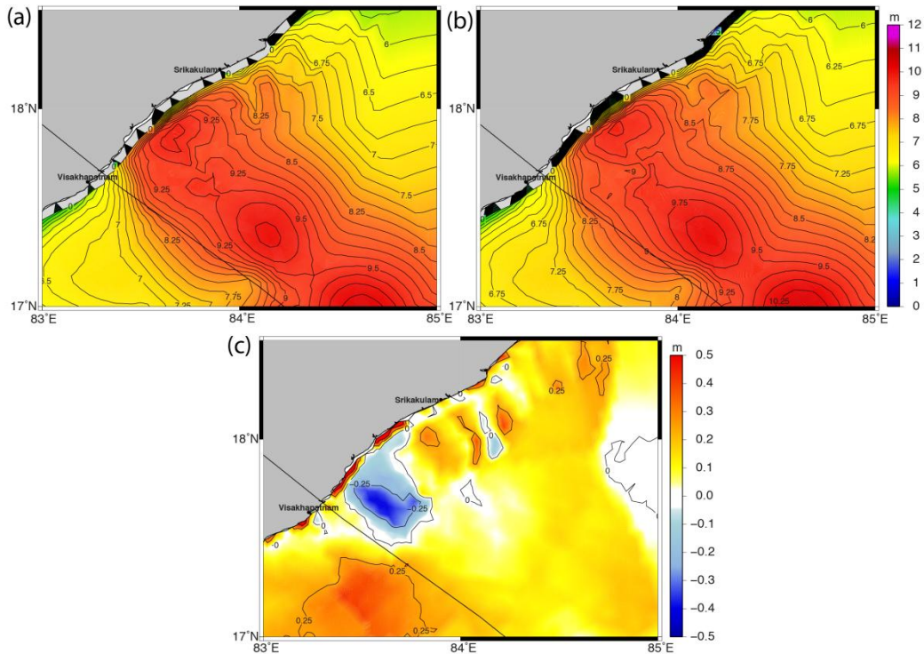
550 Fig.10. Spatial distribution of maximum significant wave heights ( H_s ) simulated along the track of Hudhud cyclone using (a) SWAN model (no wave-current interaction), (b) coupled ADCIRC+SWAN model (with wave-current interaction); colour code and contours represent H_s ; (c) change in H_s from (a) and (b), illustrating change in wave energy due to wave-current interaction.
