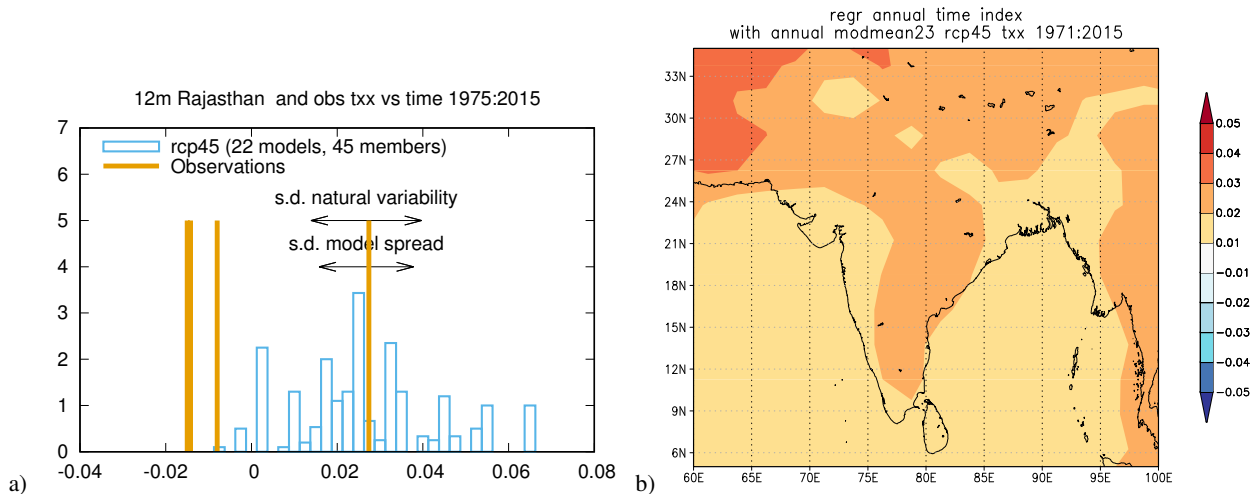
Figure 9. a) Histogram of the trend in TXX (K/yr) at the grid point closest to 26°N, 73°E in the CMIP5 ensemble (excluding the MIROC models). Ensemble members of the same model are downweighted so that each model gets weight one. This is compared with observations: the trends in Bikaner (corrected for varying missing data), Jodhpur and the nearest grid point of the ERA-interim reanalysis (left three bars). For reference the trend in the IMD gridded dataset without correction for varying missing data is also given (right-most bar). b) Mean of trend in TXX (K/yr) in the CMIP5 ensemble 1971–2015, with historical experiments up to 2005 extended with the RCP4.5 simulations 2006–2016.
