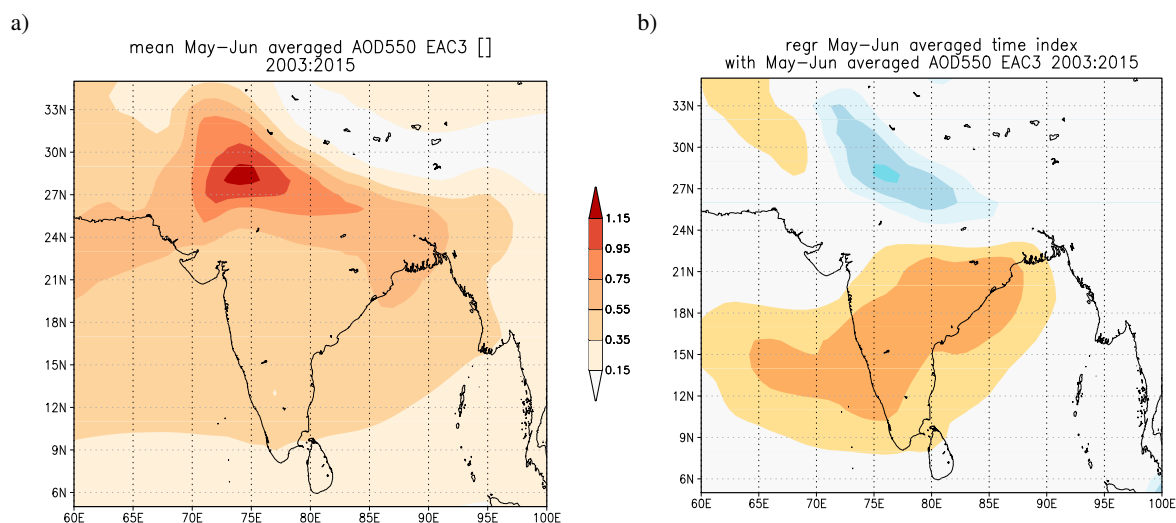
Figure 7. a) Mean May–June aerosol optical depth at 550 nm (AOD550) in the EAC3 reanalysis 2003–2015. b) Trend in AOD550 over this period ( \text{yr}^{-1} ).
