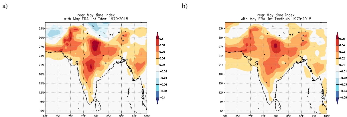
Figure 8. Trend in a) dew point temperature and b) wet bulb temperature in ERA-interim over May (K/yr).
