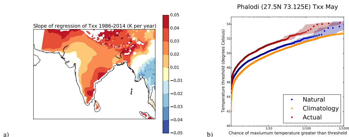
Figure 10. a) HadRM3P model trend 1986–2014 of TXx in May (K/yr). Ocean points and areas not significant at p < 0.05 are shown as white. b) Return time plots for TXx in May at the grid box closest to Phalodi, for Actual 2016 simulations (red), Natural 2016 simulations (blue) and Climatology 1986–2014 simulations (yellow).
