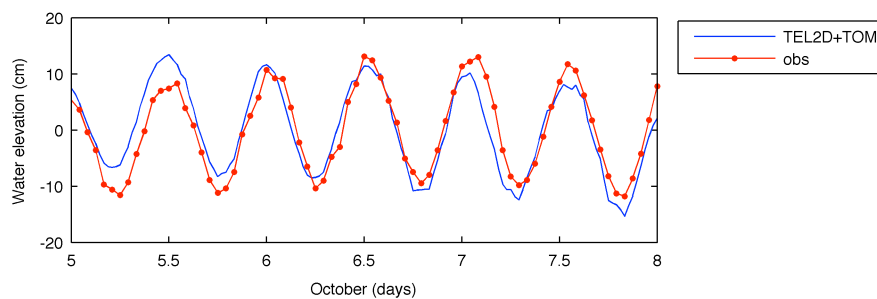
Figure 4. Time series of the tidal water elevation at the Mar Grande station: numerical results from the coupled TEL2D+TOM run (blue line) and observations (red circles).
