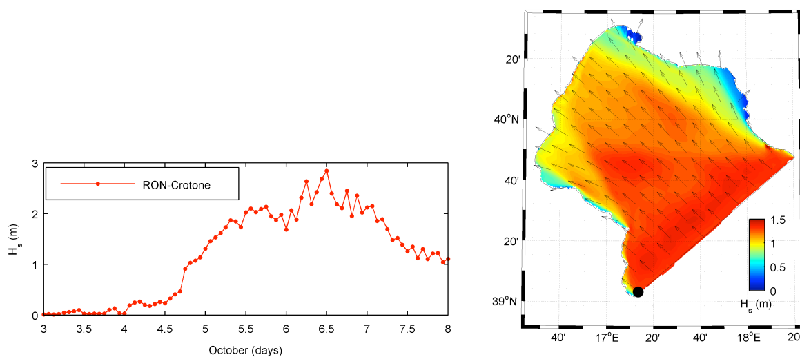
Figure 5. Numerical results from the TEL2D+TOM run for the Gulf of Taranto: significant wave height from Crotone buoy (black circle) imposed on the offshore model boundary (left panel), and snapshot (right panel) of wave propagation on 6 October 2014 at 2:00 pm (colormap of the significant height H_s and arrows of the mean direction).
