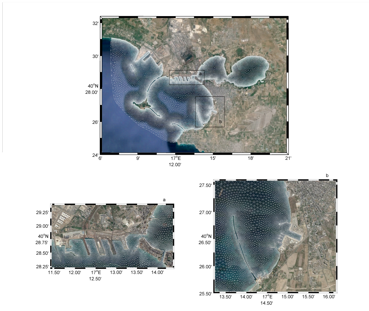
Figure 7. 3D model of the Taranto Sea: the overall grid (top panel) and two detailed zones (bottom panels) close to the Commercial Harbor (a) and the Military Harbor (b) of Taranto; background images are from Google Earth, 2016, privately processed.
