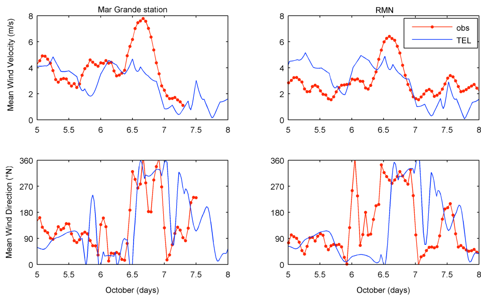
Figure 3. Wind characteristics at Mar Grande (left panels) and RMN (right panels) stations: velocity magnitude (top panels) and direction (bottom panels) from the interpolated-COSMO-ME values on the TELEMAC grid (blue line) and from observations (red line, circle markers).
