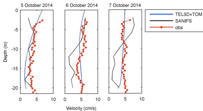
Figure 12. Daily-averaged vertical profile of current at the Mar Grande station: numerical results from the coupled TEL3D+TOM (blue line), SANIFS (black lines) and observations (red line-circle markers).
