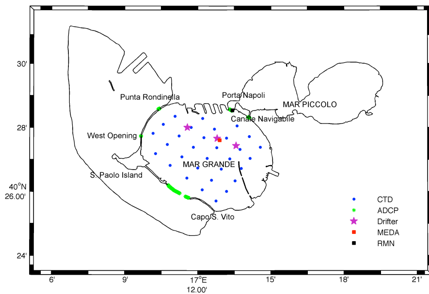
Figure 2. Map of the Mar Grande study area and points/locations of available measurement data sets from MREA14 campaign (CTD, ADCP, and drifters), the Italian Mareographic Network (RMN) and the Mar Grande station (MEDA).
