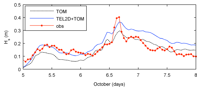
Figure 6. Significant wave height H_s at the Mar Grande station: numerical results from the standalone TOM run (black line), the coupled TEL2D+TOM run (blue line) and observations (red circles).
