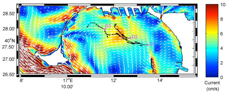
Figure 9. Surface velocity in the area of Mar Grande on 5 October 2014 (average over 10:00 am-12:00 pm): numerical results from coupled TEL3D+TOM (colormap for the velocity magnitude and white arrows for directions) and drifter routes (in black arrows).
