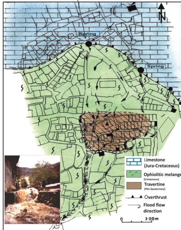
Figure 5. Map of flooding road in Sütcüler settlements (modified by Karagüzel 1998)
