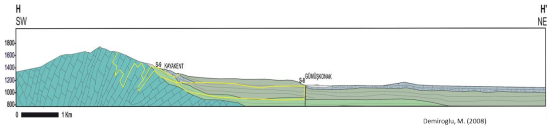
Figure 3 a) Gunyuzu marbles b) The geological cross- section of Gunyuzu springs (Demiroğlu 2008)
