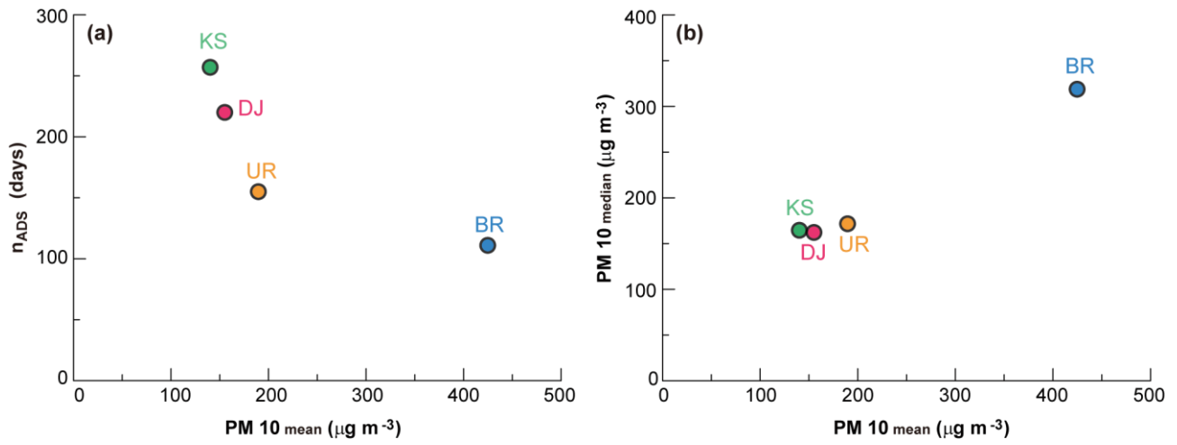
Figure 8: (a) An inverse correlation between ADS occurrence ( n_{\text{ADS}} ) and annual mean PM10 dust air concentration ( \text{PM10}_{\text{mean}} ). (b) A positive correlation between median PM10 dust air concentration ( \text{PM10}_{\text{median}} ) and annual mean PM10 dust air concentration ( \text{PM10}_{\text{mean}} ).
