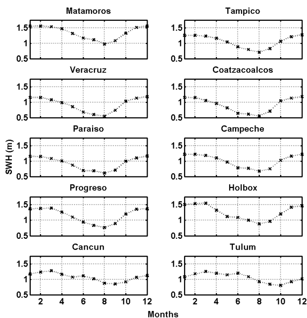
Fig. 2. Monthly mean SWH for each studied node.
