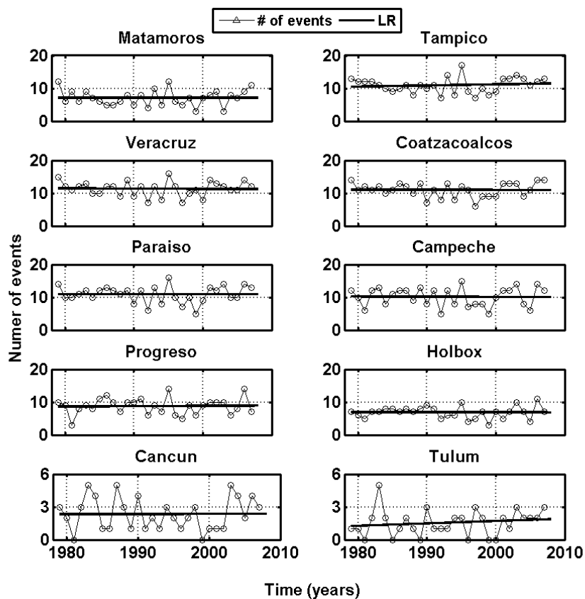
Fig. 5. Number of events caused by Nortes per season. Simple linear regressions for the data are shown, with the values of the slopes of the regression lines given in Table 2. Notice the different vertical scale used for the Cancun and Tulum nodes.
