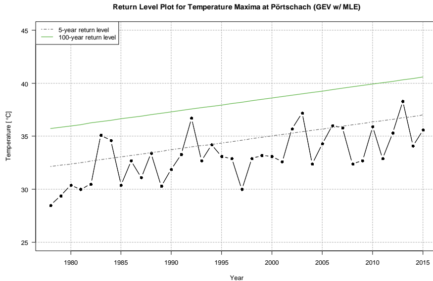
Figure 2: Return level plot of temperature maxima at Pörschach (Carinthia) with linear trend correction. The trend is visible in the lines depicting the 5-year return level (gray dashed line) and the 100-year return level (green solid line). This is an illustrative example of temperature trends that are commonly observed at the selected stations for both temperature maxima (increasing trend) and temperature minima (decreasing trend).
