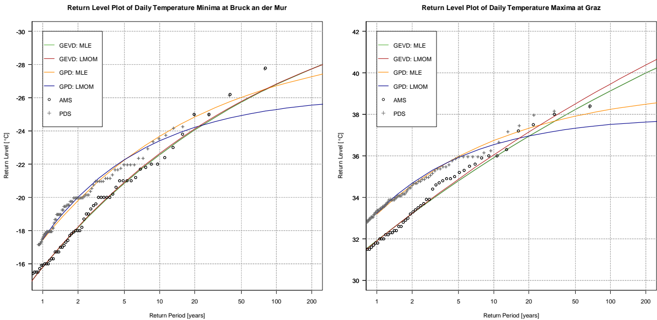
15 Figure 7: Return level plots of (a) temperature minima at Bruck an der Mur , and (b) temperature maxima at Graz . Return level estimation is based on the block maxima approach and on the threshold excess approach with two different parameter estimation methods (MLE and LMOM-estimation).
