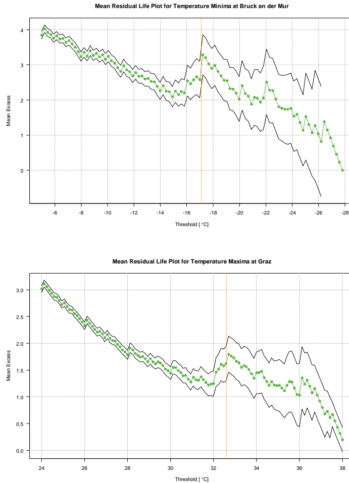
Figure 8: Mean residual life plots of (a) temperature minima the hot spot in Bruck an der Mur and (b) temperature maxima at Graz . Black lines indicate the 95% confidence interval for the mean excess and orange lines indicate the threshold selected by means of the square root rule.
