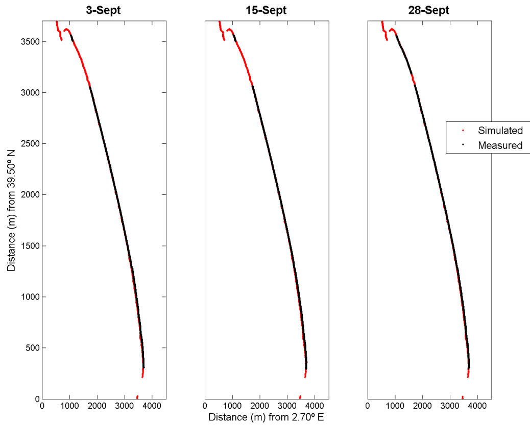
Figure 132. Observed (black) and modelled by SWASH (red) shoreline positions in Playa de Palma
