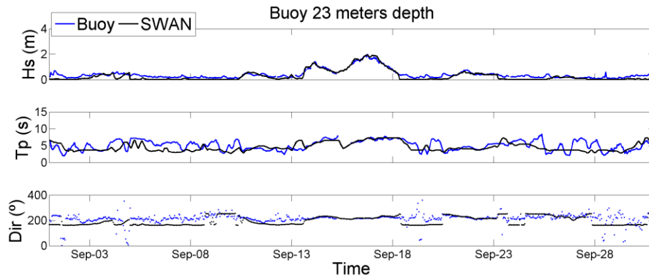
Figure 910: Hs, Tp and wave direction as modelled by SWAN model and observed at the buoy deployed at 23 m depth in Playa de Palma beach.
