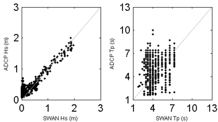
Figure 101: SWAN vs ADCP scatter plots of Hs (left) and Tp (right) in Playa de Palma.
