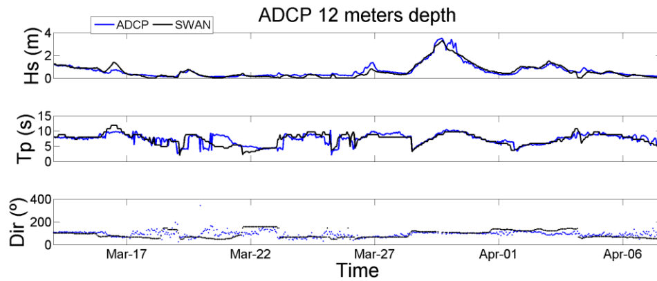
Figure 87: Hs, Tp and wave direction as modelled by SWAN and observed at the ADCP deployed at 12m depth in Cala Millor beach.
