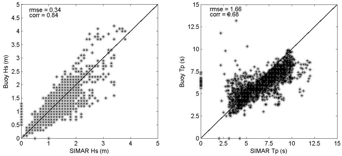
Figure 7:6 Scatter plots of buoy observations vs SIMAR hindcast for Hs (left) and Tp (right). RMSE and correlation are quoted in each figure.
