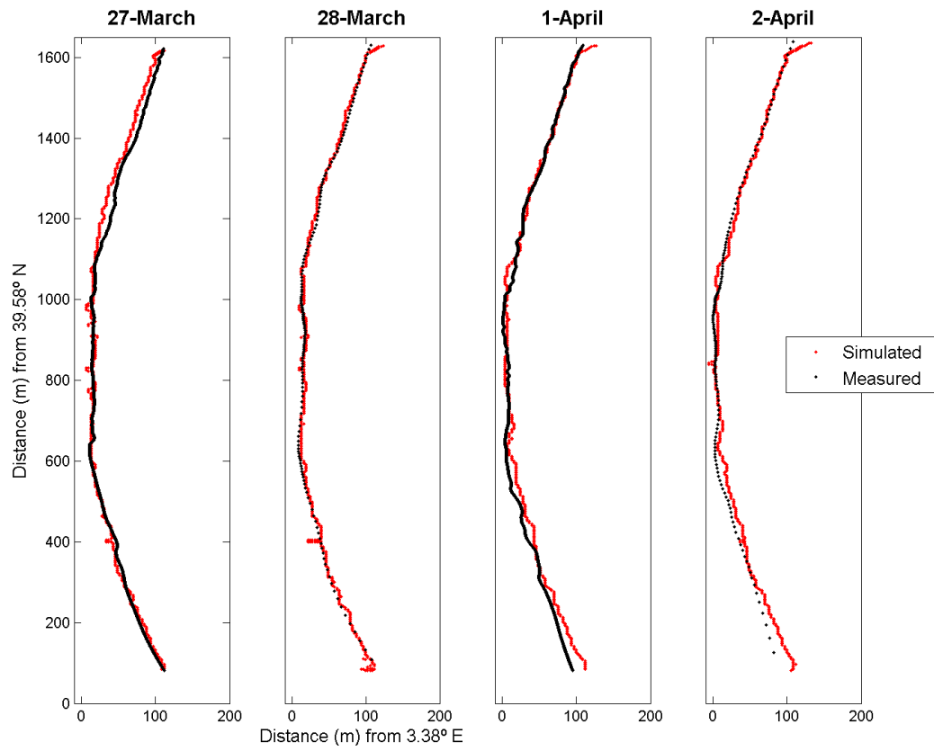
Figure 4.12. Observed (black) and modelled by SWASH (red) shoreline positions in Cala Millor
