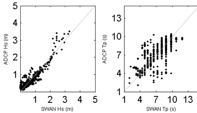
Figure 89: SWAN vs ADCP scatter plots of Hs (left) and Tp (right) in Cala Millor.
