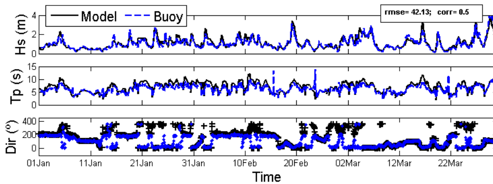
Figure 6: Capdepera buoy observations (blue) and hindcasted SIMAR (black) time series of H_s , T_p and wave direction. RMSE and correlation are quoted for the wave direction (for H_s and T_p the values are quoted in Figure 6).
