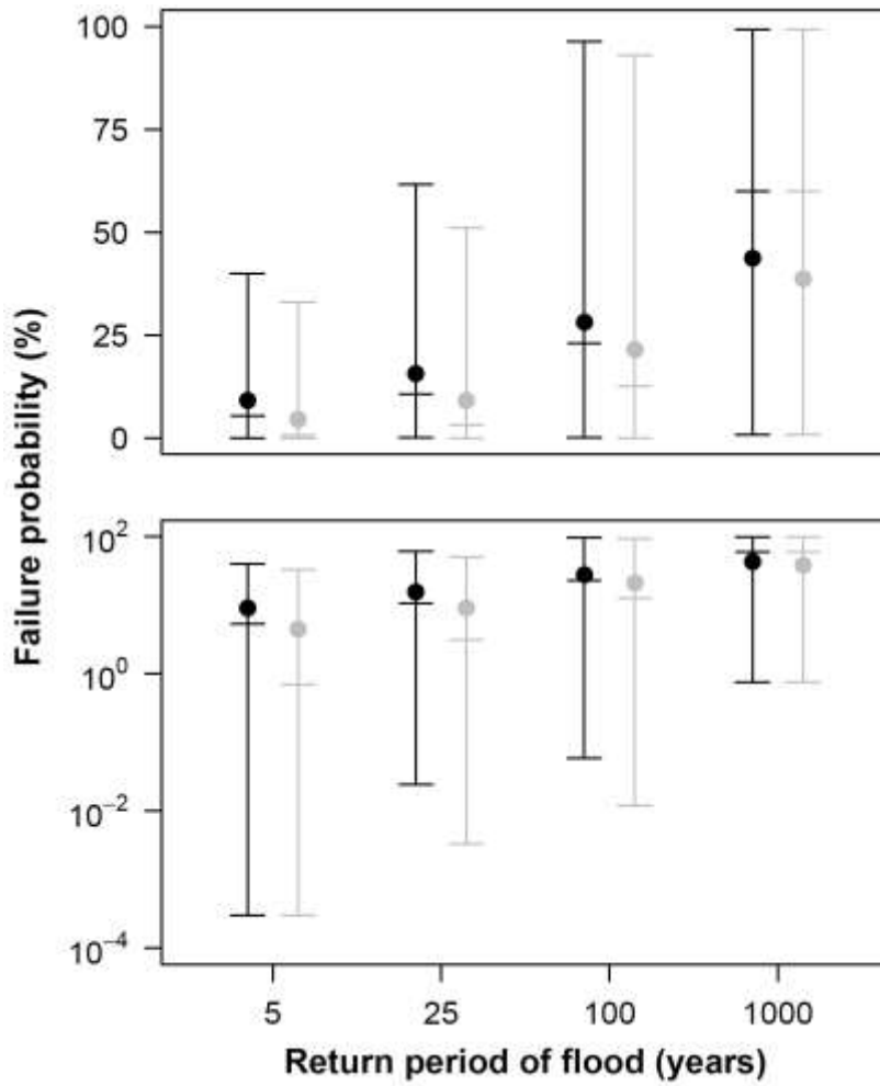
Figure 5. Estimated bridge failure probabilities as a function of flood event severity, expressed in terms of the return period of the flood event , conditional on a preceding flood event of 100-year return period having occurred with no intervening maintenance action. Upper and lower panel show the same data, plotted on different scales.
