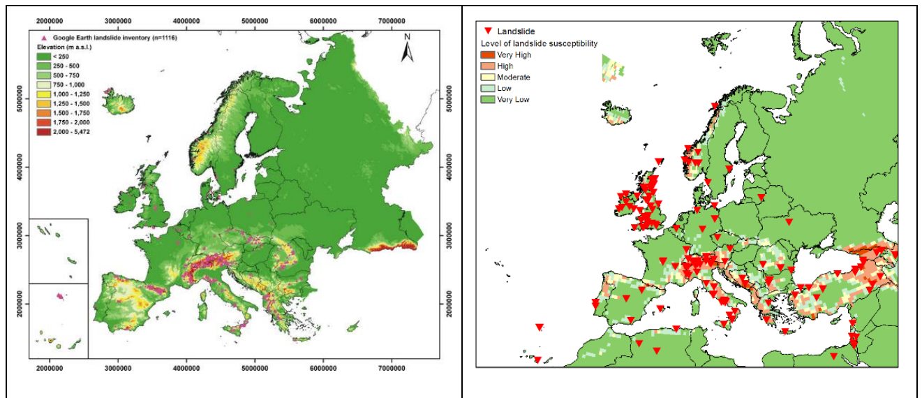
1 Fig.2 Comparison of landslide overlay in this research and that in existing study
