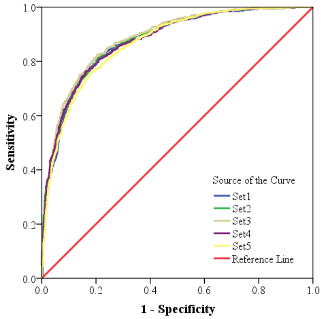
1 Fig.3 ROC curve of modeling process
