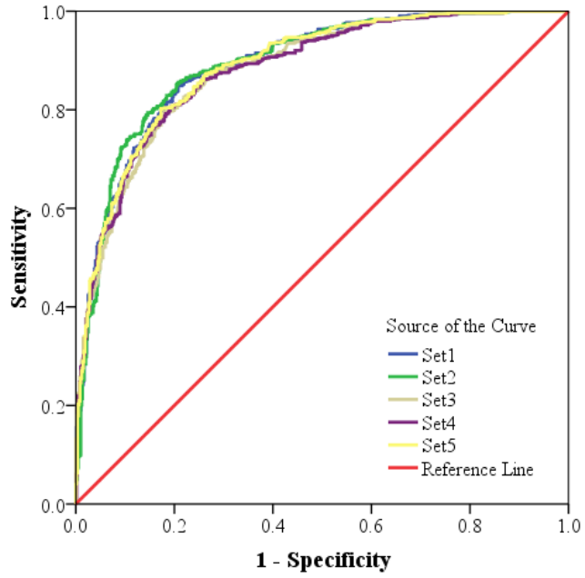
1 Fig.4 ROC curve of validation process 2
