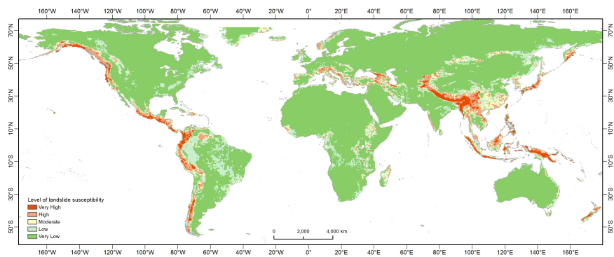
Fig. 2. Global scale landslide susceptibility map
