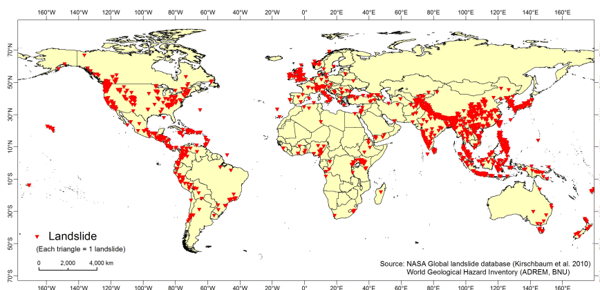
Fig. 1. Landslide location in the combined landslide database
