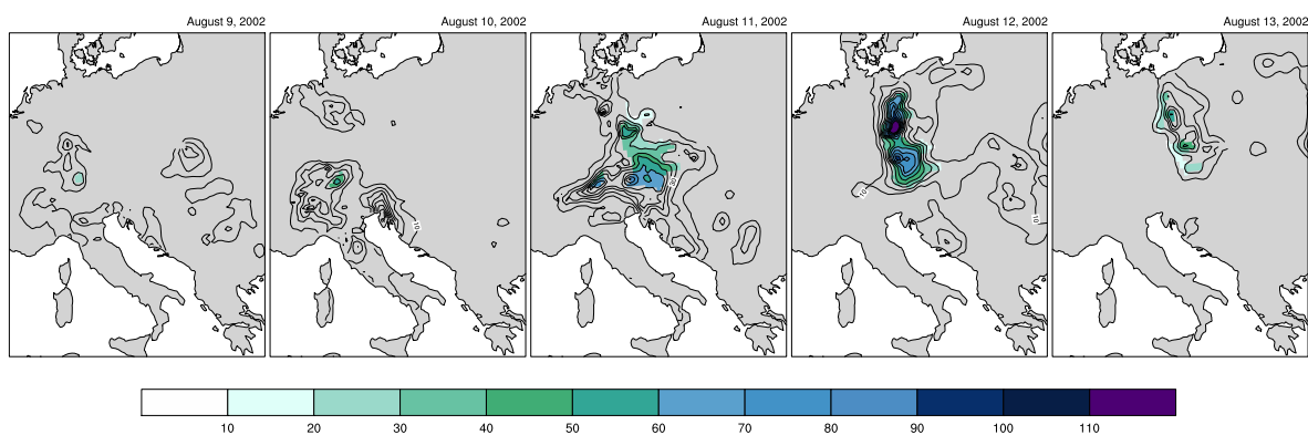
Figure 3. Precipitation for the period August 9 2002 to August 13 2002 based on the E-OBS data set. Contour lines show daily precipitation amounts. Colour denotes grid boxes in which the local 10-year return levels are exceeded. Units mm.
