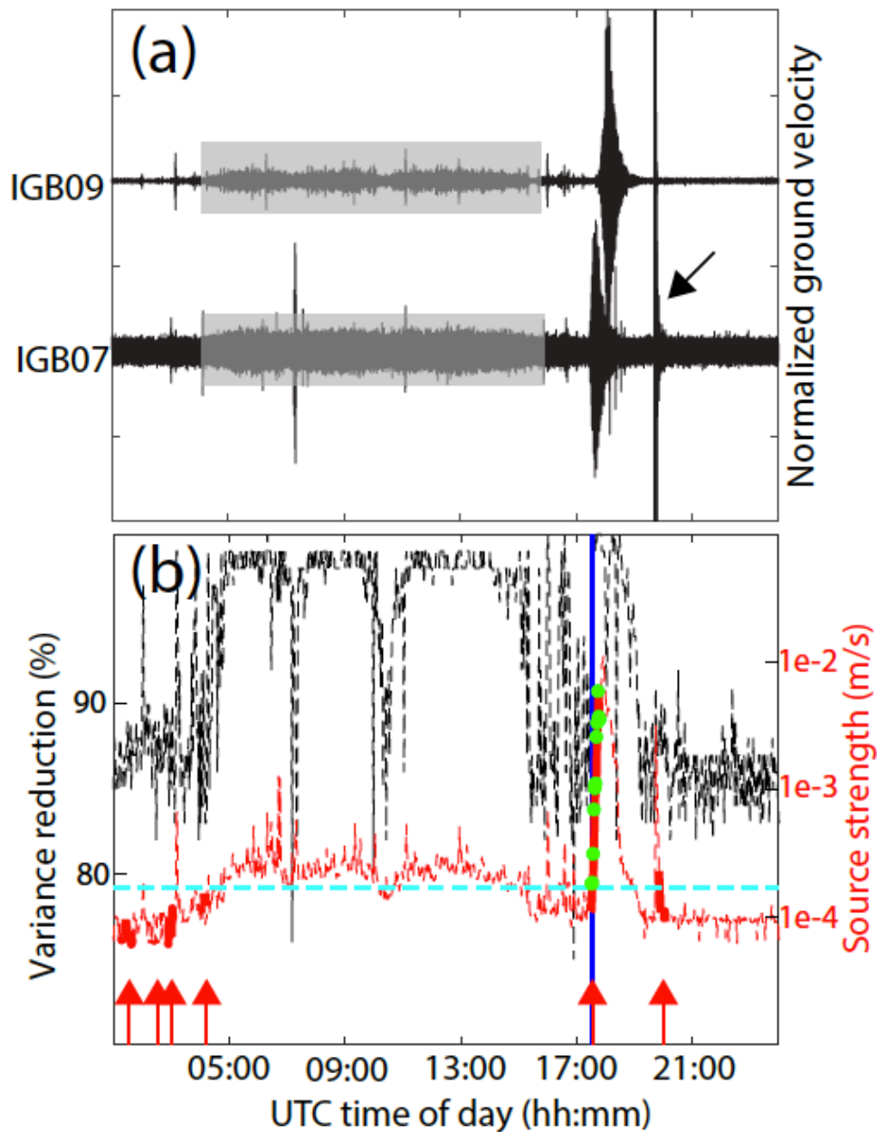
Figure 9: Results of the ASL approach . (a) Seismograms of stations IGB07 (in the Illgraben catchment) and IGB09 (in the Rhone Valley). Black arrow indicates high-frequency arrivals of the M6.2 2011 Fergana Valley earthquake in Kyrgyzstan. Grey boxes highlight increased amplitudes due to anthropogenic noise. (b) Variance reduction (black) and equivalent source strength (red). Thick solid red lines denote time instances when the best fit location lies in the Illgraben catchment (also indicated with red arrows), dashed lines denote the remaining time instances. Green dots represent times when three detection criteria were satisfied: (1) location in upper catchment, (2) variance reduction above 90 % and (3) source strength A_0 above 1.7e-4 m/s. The blue vertical line marks 17:32, which we propose as the initial detection time of the debris flow.
