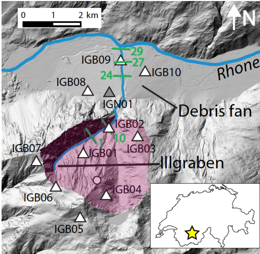
Figure 1: Illgraben region with its upper catchment area (shaded polygon) and debris fan in the Rhone Valley. Numbered green lines represent Check Dams 1, 10, 24, 27 and 29; 2011 seismometer locations are indicated by triangles (grey triangle represents the 2015 noise record station) and a WSL rain gauge is indicated by the circle. Inset shows outlines of Switzerland and yellow star marks location of Illgraben.
