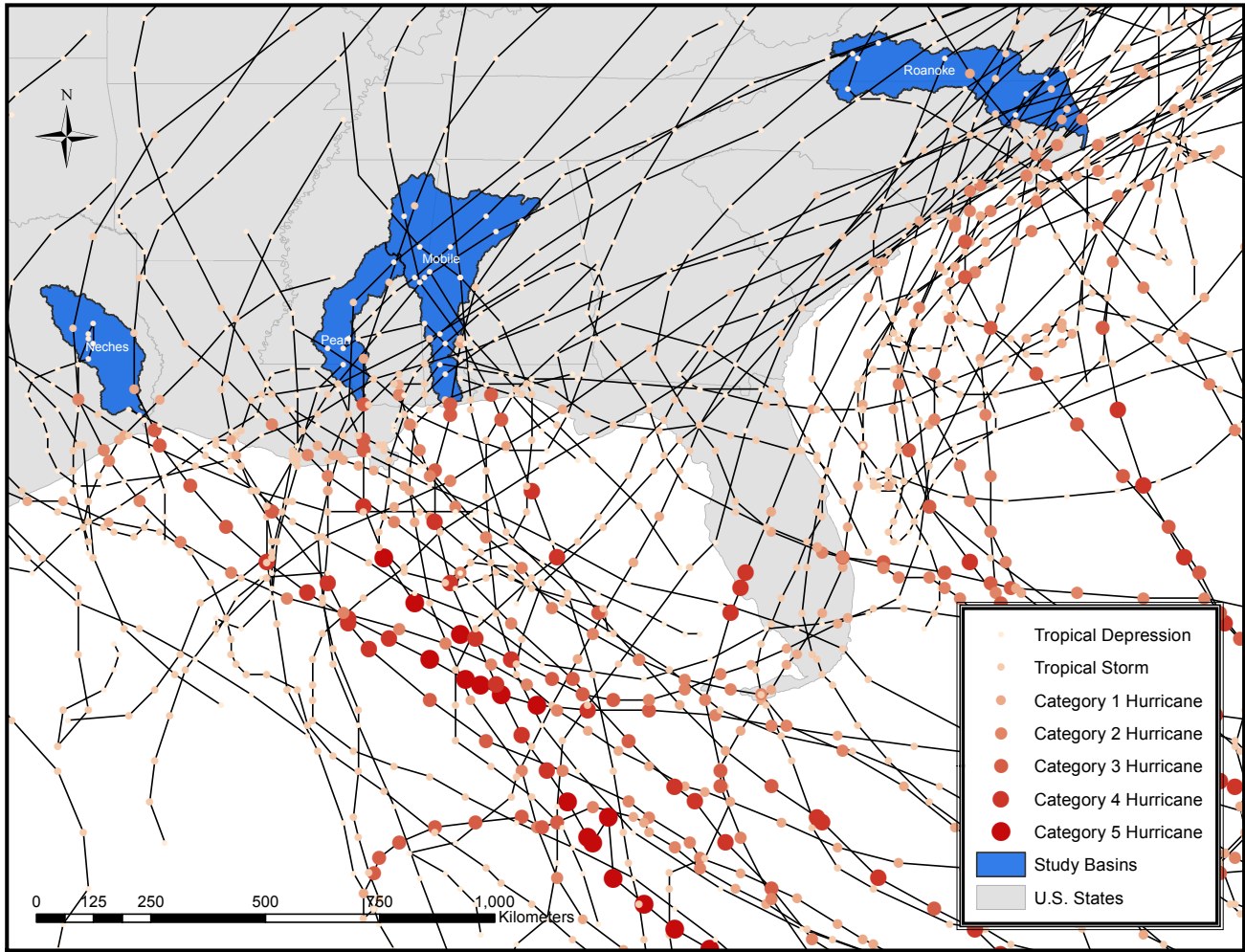
5 Figure 1: Location of the study basins analyzed in this study (blue); colored dots represent points along the tracks of all tropical cyclones since 1998 that impacted the study basins, where the color/size of the dot indicates the severity of the storm at that location (see legend). (HURDAT2, NHD, ESRI)
