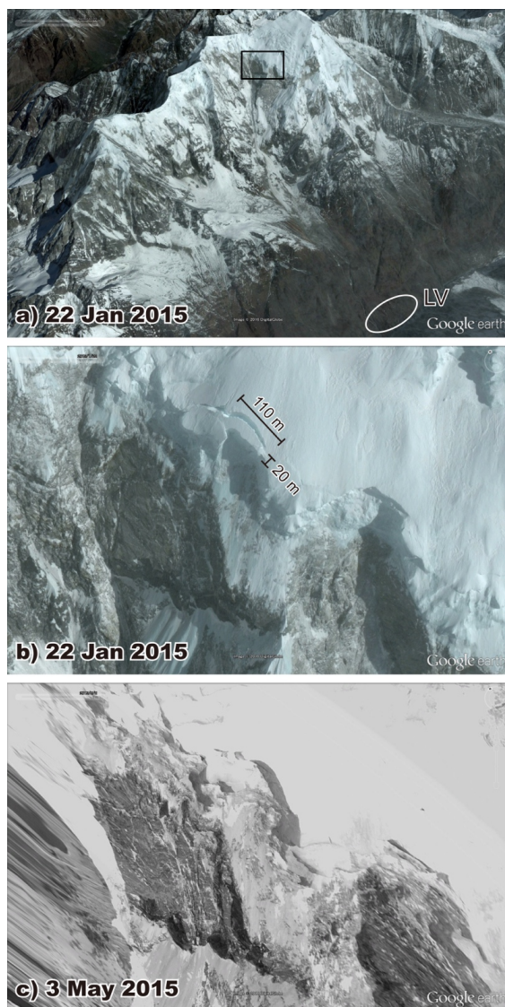
Figure 12: An example of collapsed glacier ice captured from the Google Earth. Panels are a) overview of the southwest face of Mt. Langtang Lirung, b) ice block found in the pre-event image on 22 January 2015, and c) the ice lost from the post-event image on 3 May 2015, respectively. Black box and ellipse in panel (a) denote area of panels (b) and (c), and the damaged Langtang village (LV), respectively.
