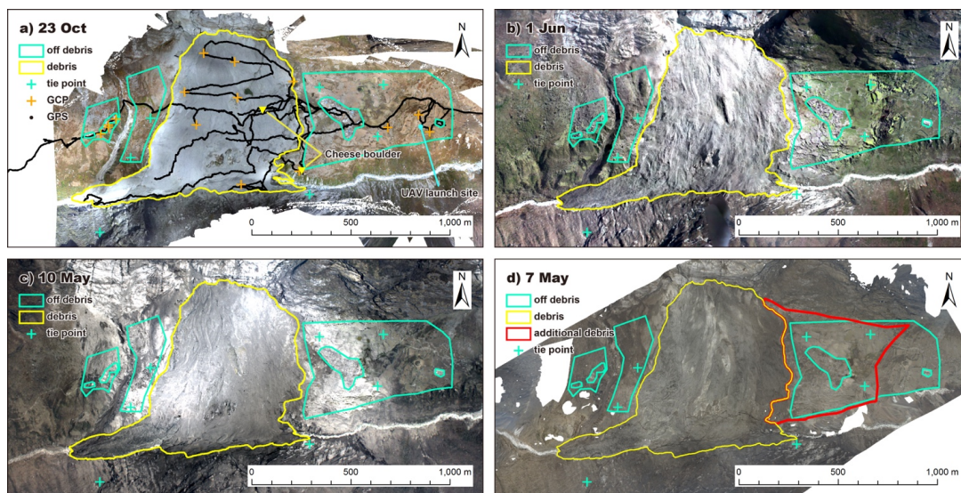
Figure 2: Orthoimages over the Langtang village on (a) 23 October, (b) 1 June, (c) 10 May and (d) 7 May of 2015.
