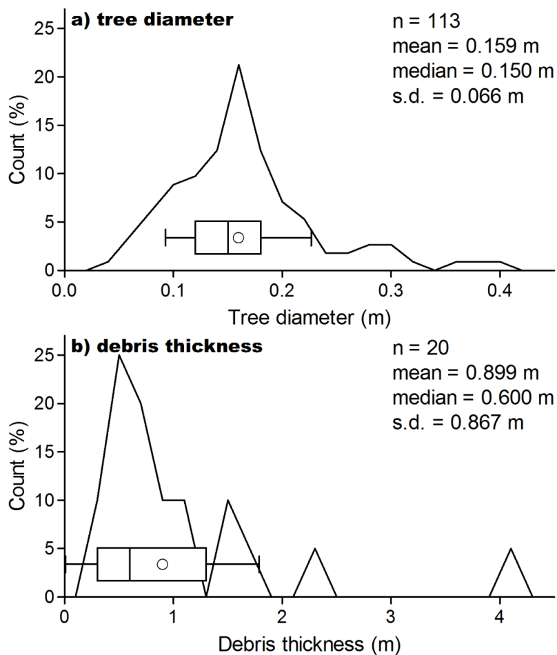
Figure 8: Histogram and box plot of (a) diameter of trees fallen on the opposite slope of the Langtang village and (b) debris thickness found at ice cliffs. Box, line and circle in box and whisker denote interquartile, median and mean, and one standard deviation, respectively.
