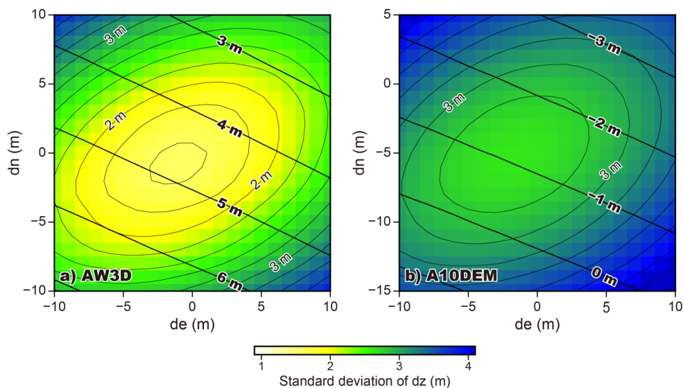
5 Figure 3: Distribution of elevation bias ( dz , thick contour lines) and its standard deviation (color shadings with thin contour lines) of (a) AW3D and (b) A10DEM against the UAV-DEM on 23 October, which are calculated over the off-debris area (Fig. 2a). ALOS-DEMs are shifted at 1-m interval to both directions of west to east ( de , horizontal axis) and of south to north ( dn , vertical axis), and then mean elevations for 5-m cells (corresponding to the ALOS-DEMs) are calculated from the UAV-DEM, which is resampled to 5-m from the original 1-m resolution.
