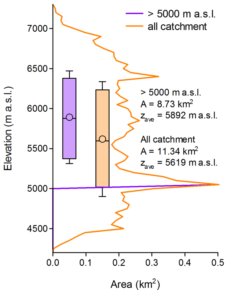
5 Figure 11: Hypsometry and box plot for the upper catchment above the Langtang village, from which the main avalanche might have occurred (orange polygon in Fig. 1). Also shown is that limited above 5000 m a.s.l. Elevation data is used from ASTER-GDEM2 (Tachikawa et al., 2011). Box, line and circle in box and whisker denote interquartile, median and mean, and one standard deviation, respectively.
