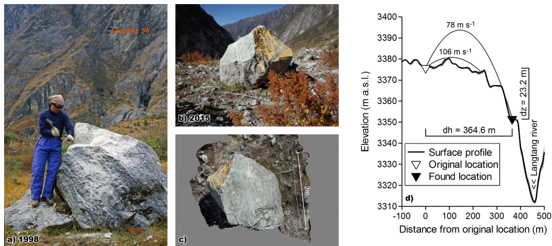
5 Figure 6: Photographs of the 'cheese boulder', (a) when the sculpture was carved in 1998, (b) during our in-situ observation (22 October 2015), and (c) screenshot from the structure from motion analysis with the similar angle of (a). (d) Cross section profile along which the boulder moved. Locations (Fig. 2a) and the surface profile were obtained by dGPS survey and the UAV-SfM products. Elevation error is calculated based on the UAV-DEM (1-m resolution) by computing a standard deviation within a 5 m distance. Thin parabolic curves denote possible passes, along which the boulder was blown. Higher curve does not touch the ground between the original and found locations while lower curve can cross the 4.5-m height hill, and then the boulder could roll down. Also shown are the initial speeds at the original location for the boulder to have the passes.
