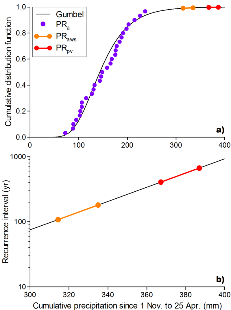
Figure 10: (a) Cumulative density function of cumulative precipitation since 1 November to 25 April ( PR_a , purple circles) and the Gumbel density functions (black line), and (b) recurrence interval. Red and orange circles denote calibrated precipitation for the elevation of Kyangjin (3830 m a.s.l.) from two sites near Yala Glacier (Fig. 1) assuming two elevation gradients for precipitation.
