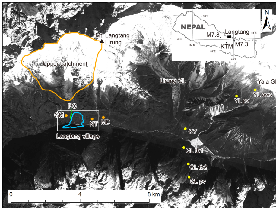
5 Figure 1: Langtang village surveyed in this study (white polygon indicating area of Figs. 2 and 5), debris covering the village (blue polygon), upper catchment from which the avalanche could have originated (orange polygon), other villages mentioned in the text (orange circles), small gorge (green line), and locations where meteorological stations are located (yellow circles) in the valley (valley location shown in inset panel). The background is based on an ALOS-PRISM image taken on 3 December 2010 before the Gorkha earthquake. Abbreviations denote GM: Gomba, PC: Pääbe Chu, NT: Numthang, MD: Mundu, KY: Kyanjin, YL: Yala, GL: Gangja La, aws: automatic weather station, pv: pluviometer, and tb: rain gauge of tipping bucket.
