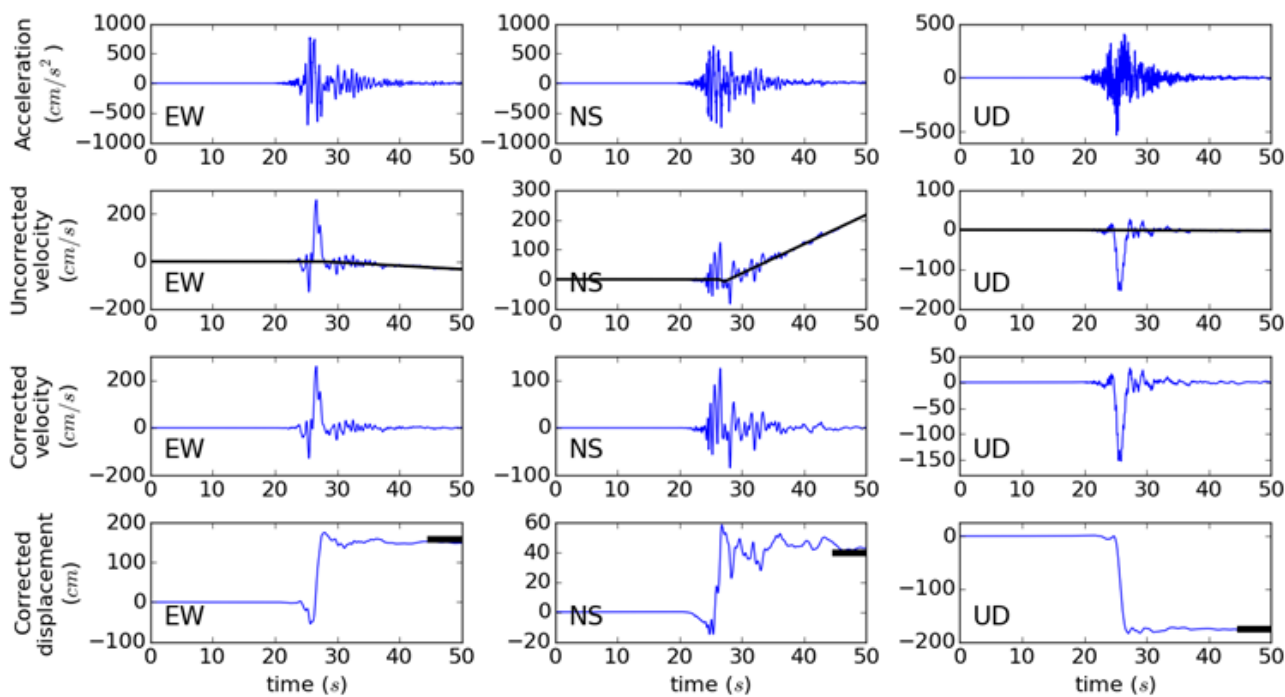
Figure 12. Example of baseline correction procedure for the acceleration recorded at the Nishihara station. The trend of the uncorrected velocity was modeled by two straight lines based on the method by Wang et al. (2011) and was removed from the record. Then, the corrected displacement was calculated by integrating the acceleration with respect to time. The thick black line in the displacement time history represents the coseismic displacement calculated from the Lidar DSMs.
