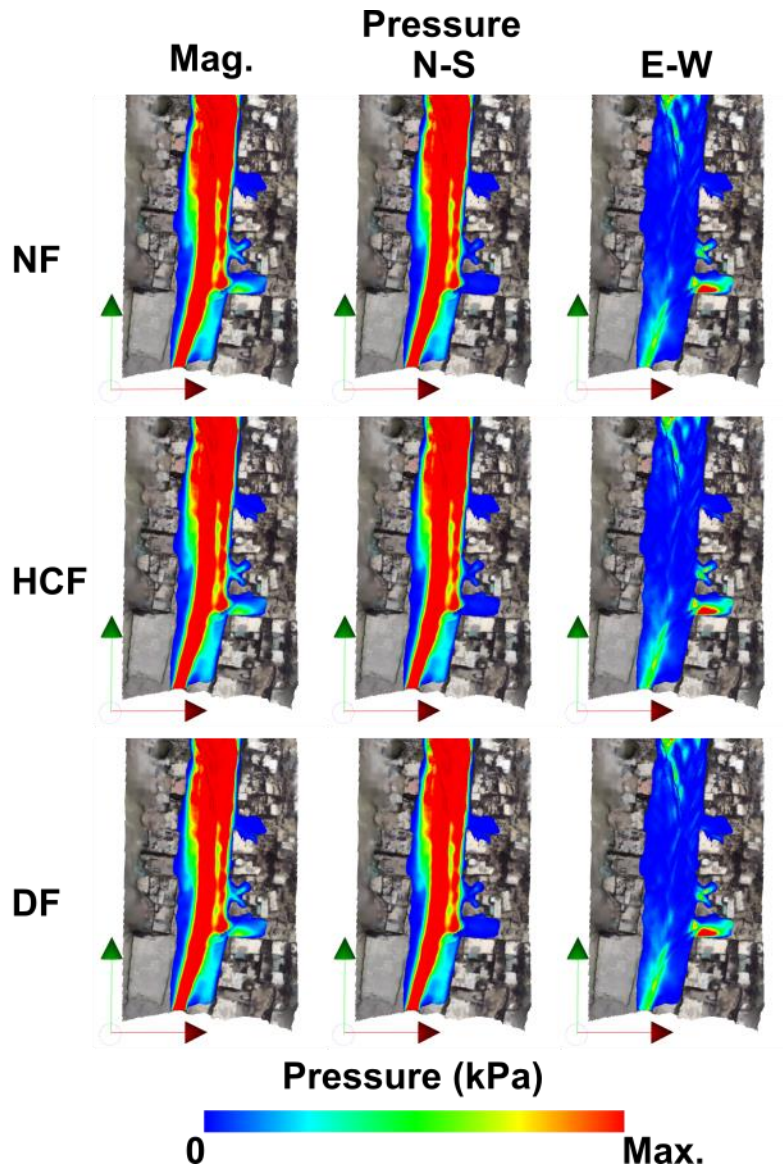
635 Figure 6. Directional components of dynamic pressure for a 75 \text{ m}^3\text{s}^{-1} flow along Quebrada Dahlia for a Newtonian flow (NF), hyperconcentrated flow (HCF) and debris flow (DF). Maximum pressure is 25 kPa for magnitude and N-S pressures, 10 kPa for E-W pressure.
