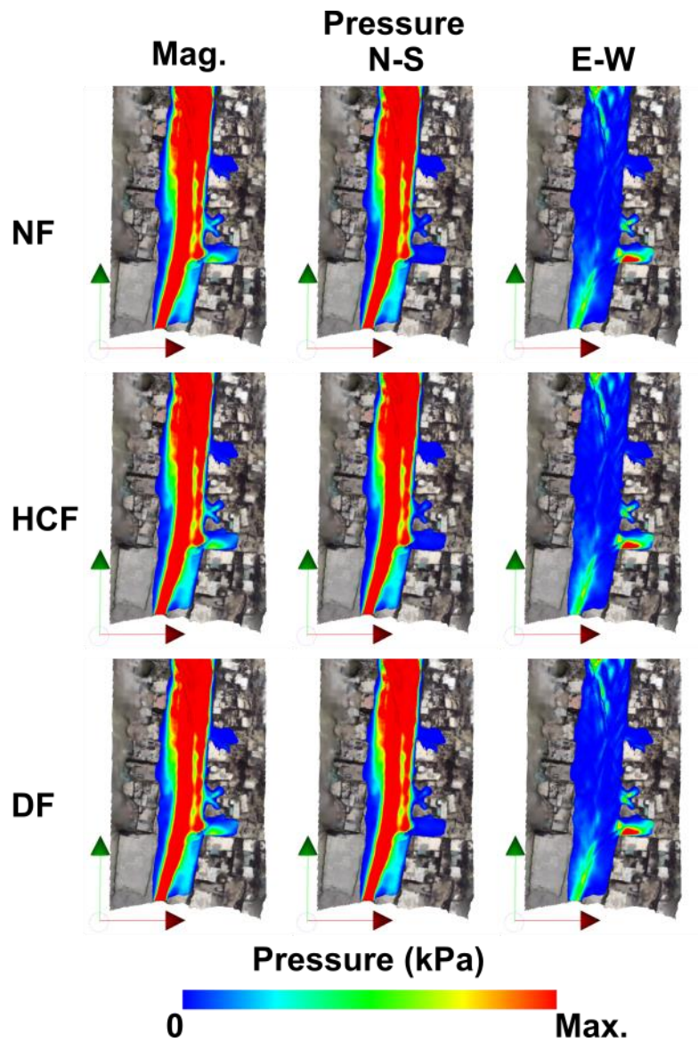
Figure 6. Directional components of dynamic pressure for a 75 \text{ m}^3\text{s}^{-1} flow along Quebrada Dahlia for a Newtonian flow (NF), hyperconcentrated flow (HCF) and debris flow (DF). Maximum pressure is 25 kPa for magnitude and N-S pressures, 10 kPa for E-W pressure.
