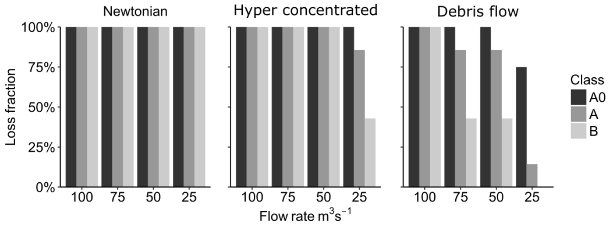
Figure 12. Building loss fraction for all flow scenarios where buildings assumed to have a brick width of 0.15 m.
