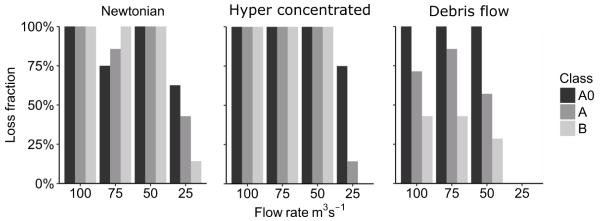
Figure 13. Building loss fraction for all flow scenarios where buildings assumed to have a brick width of 0.25 m.
