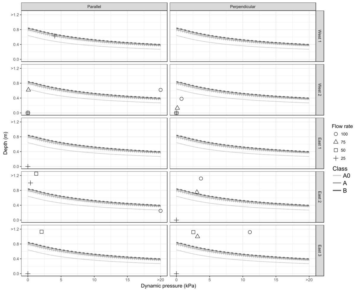
655 Figure 11. Critical depth-pressure curves for building classes A0, A and B subjected to a debris flow. Peak normal pressures and corresponding depths applied to each city block are plotted as points for each flow rate.
