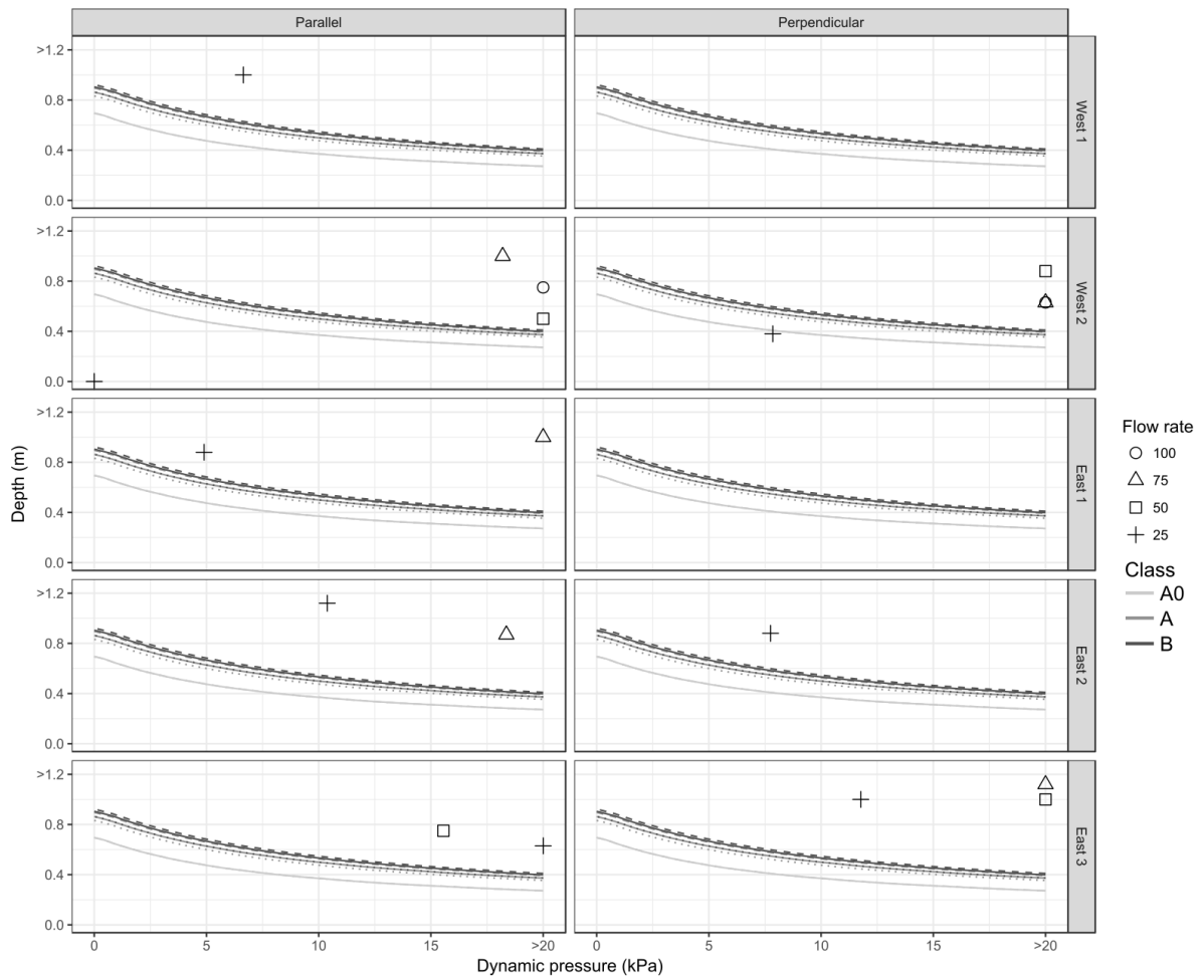
650 Figure 10. Critical depth-pressure curves for building classes A0, A and B subjected to a hyperconcentrated flow. Peak normal pressures and corresponding depths applied to each city block are plotted as points for each flow rate.
