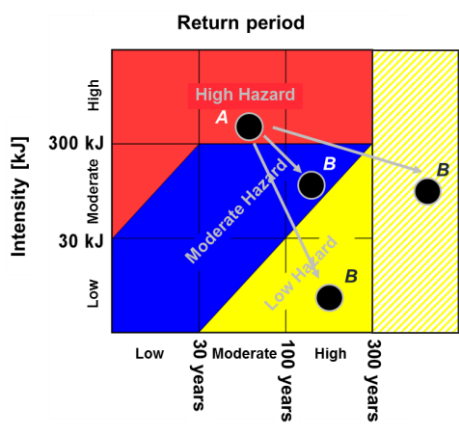
Fig. 109. Example of possible hazard reclassification at a given location of the slope, starting from a natural scenario characterised by high hazard.
