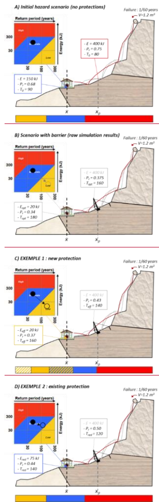
5 Fig. 9. Example of application of the methodology. A) Hazard scenario before protections; B) theoretical hazard scenario obtained in presence of the protection based on raw rock fall simulation results; C) Methodology applied for new protections: reclassification of hazard possible; D) Methodology applied for existing protections: reclassification of hazard not possible. Below each scheme the corresponding hazard zoning is reported: for cases C) and D) this is obtained by applying the methodology to every abscissa beyond the rock fall barrier.
