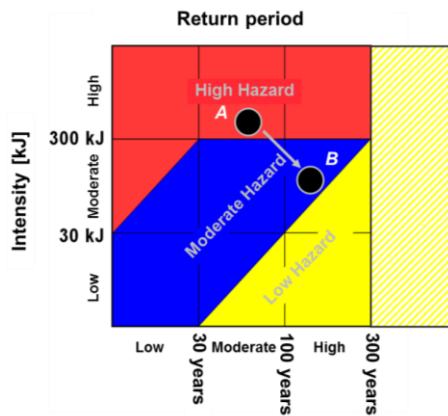
Fig. 6. Reclassification of hazard at a given location of the slope, using the Swiss intensity-frequency diagram. Point A: natural rock fall hazard scenario; Point B: new hazard level assessed once the effect of a given protection measure is taken into account.
