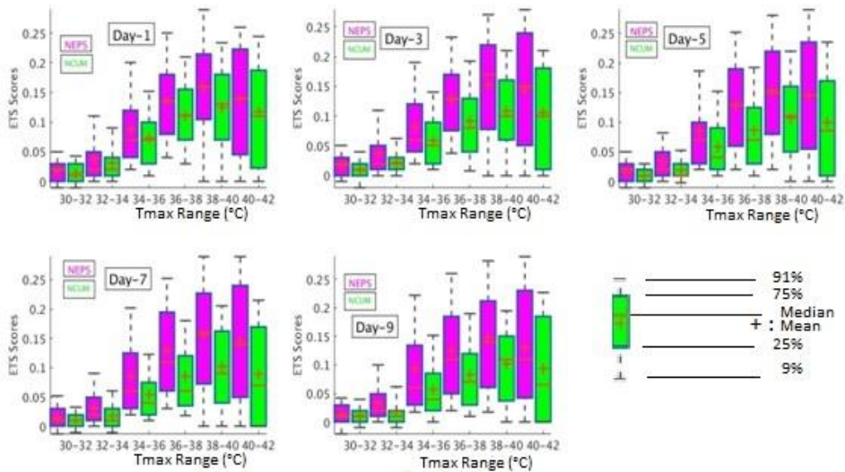
Figure 10. Box plots for Equitable Threat Score (ETS) for NCUM and NEPS from March to May 2016. (NCUM stand for NCMRWF Unified Model and NEPS stands for NCMRWF Ensemble Prediction System)
