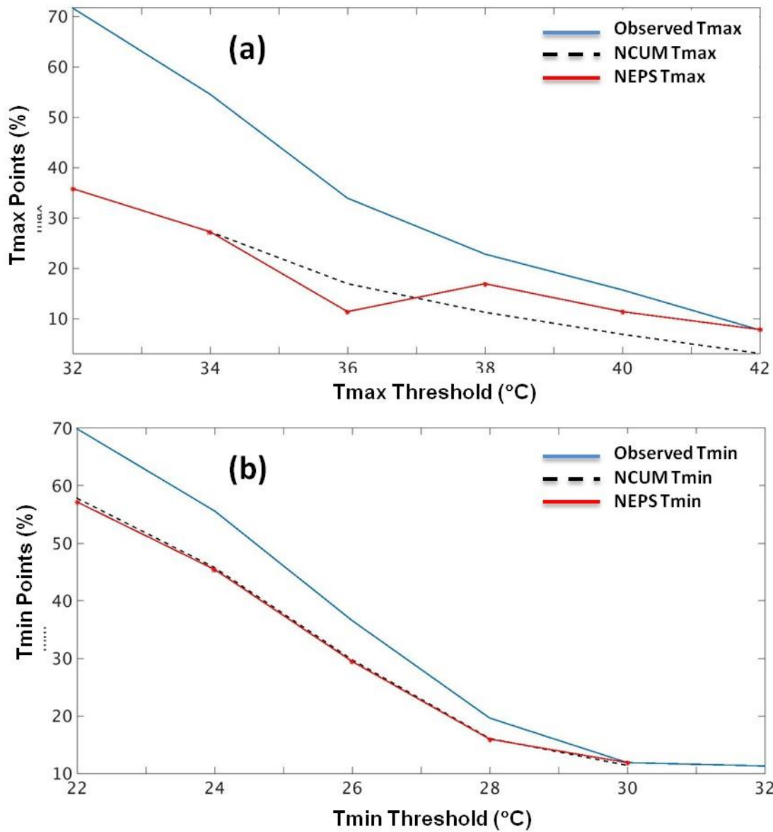
Figure 1. Frequency distribution of observed, and forecast (NCUM and NEPS) (a) T_{max} ( ^{\circ}\text{C} ) and (b) T_{min} ( ^{\circ}\text{C} ) over India during March-May 2016. (NCUM stand for NCMRWF Unified Model and NEPS stands for NCMRWF Ensemble Prediction System) [Observed data from India Meteorological Department and forecast data from NCMRWF]
