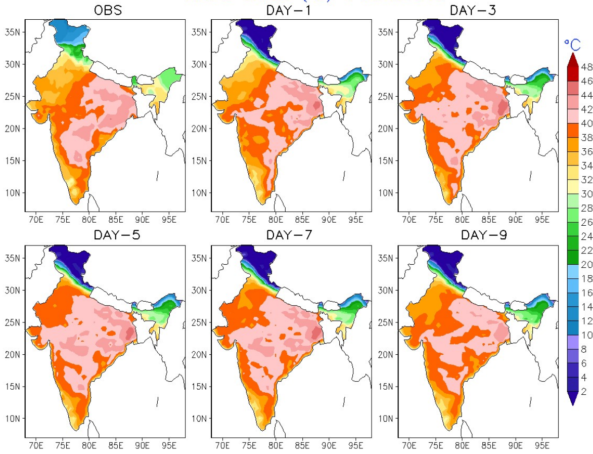
Figure 6. Spatial distributions of Observed T_{max} and NEPS forecast T_{max} prevailing heat-waves over, MP, Odisha, AP, Telangana and some parts of Maharashtra on 11 th April 2016
