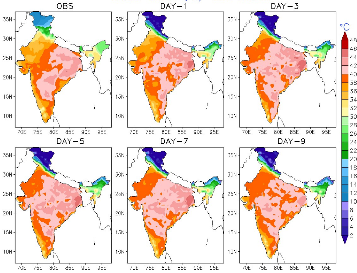
Figure 5. Spatial distributions of Observed T_{max} and NCUM forecast T_{max} prevailing heat-waves over, MP, Odisha, AP, 5 Telangana and some parts of Maharashtra on 11 th April 2016
