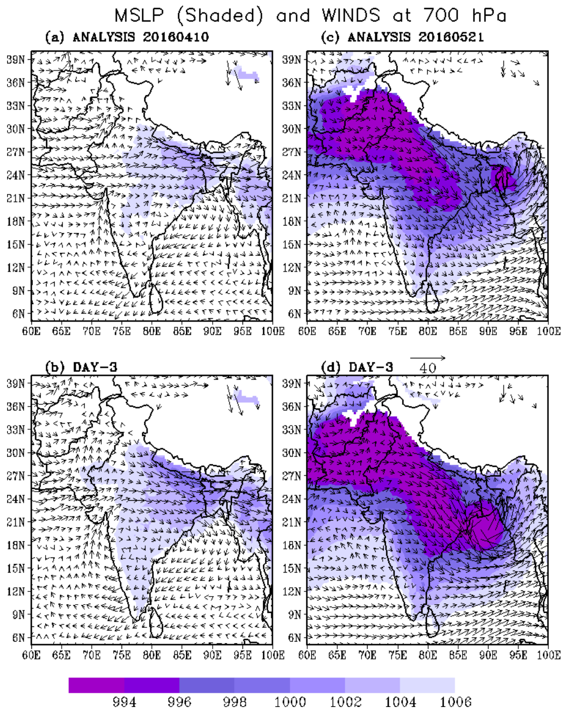
Figure 4. Mean Sea Level Pressure (MSLP) shaded and winds at 700 hPa showing heat low (a) Analysis of 20160410 (b) Day 3 forecast valid for 20160410 (c) Analysis of 20160521 (d) Day 3 forecast valid for 20160521
