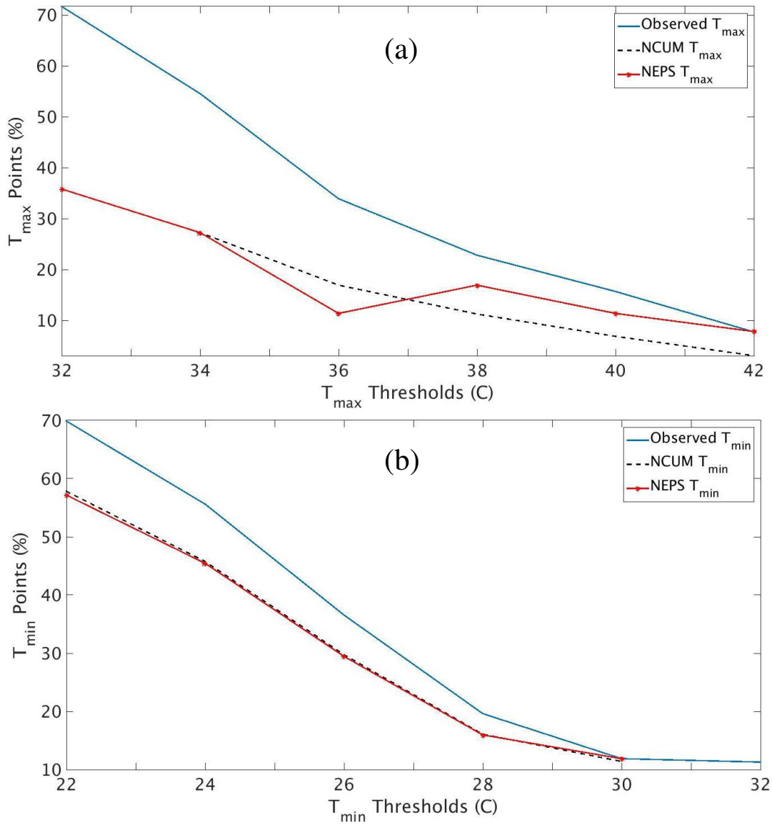
Figure 1. Frequency distribution of observed, and forecast (NCUM and NEPS) (a) T_{max} ( ^{\circ}\text{C} ) and (b) T_{min} ( ^{\circ}\text{C} ) over India during March-May 2016.
