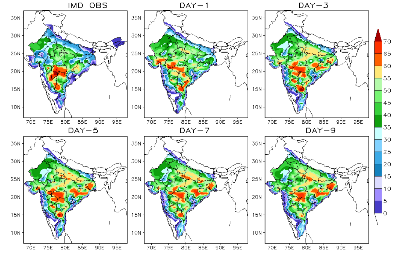
Figure 3. Spatial distribution of observed and NEPS forecasts number of days with T_{max} \geq 40^{\circ}\text{C} during the period of March to May 2016
