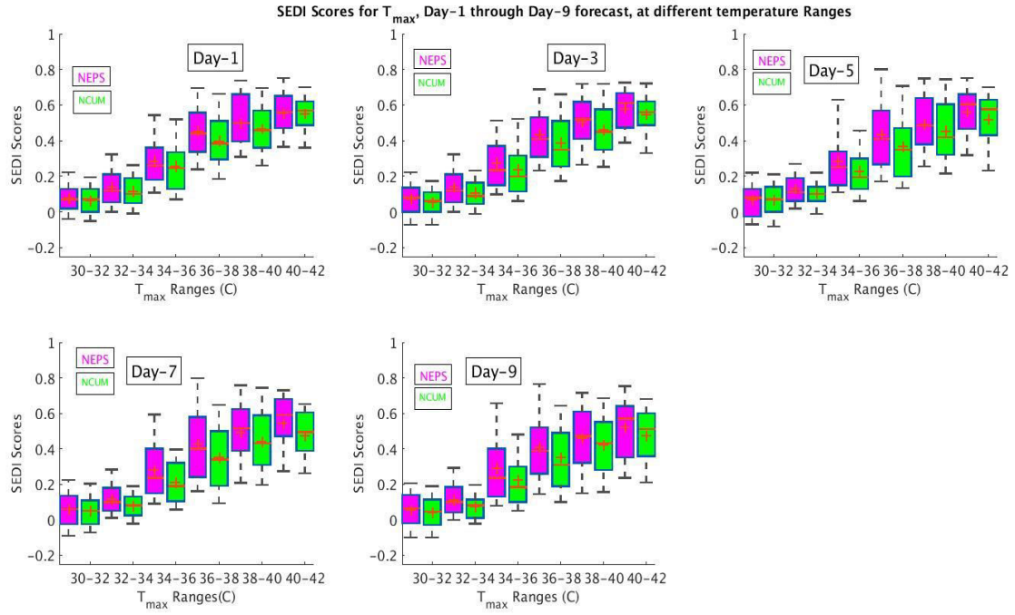
Figure 13. Box plots for Symmetric External Dependence Index (SEDI) for NCU and NEPS form March to May 2016
