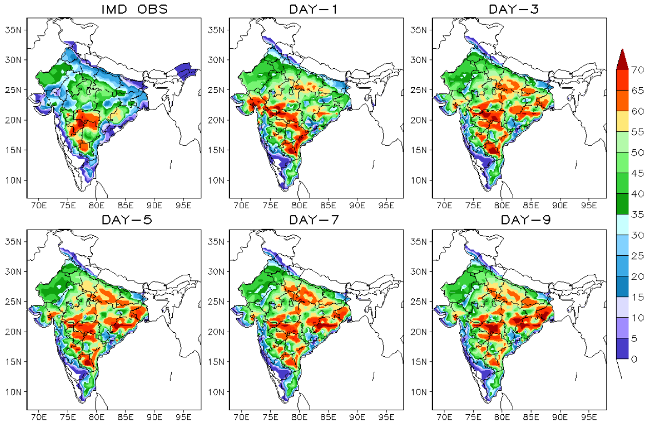
Figure 2. Spatial distribution of observed and NCUM forecasts number of days with T_{max} \geq 40^{\circ}\text{C} during the period of March to May 2016
