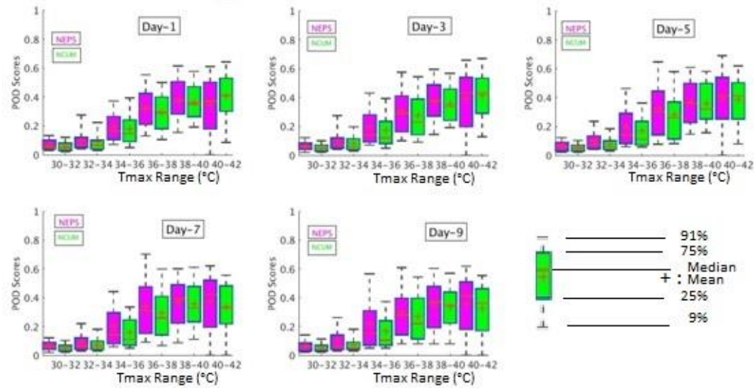
5 Figure 12. Box plots for Probability of Detection (POD) for NCUM and NEPS from March to May 2016. (NCUM stand for NCMRWF Unified Model and NEPS stands for NCMRWF Ensemble Prediction System)
