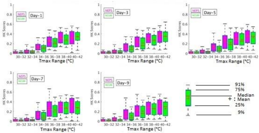
Figure 9. Box plots for HK scores for different temperature ranges ( T_{max} ) NCUM and NEPS from March to May 2016. (NCUM stand for NCMRWF Unified Model and NEPS stands for NCMRWF Ensemble Prediction System)
