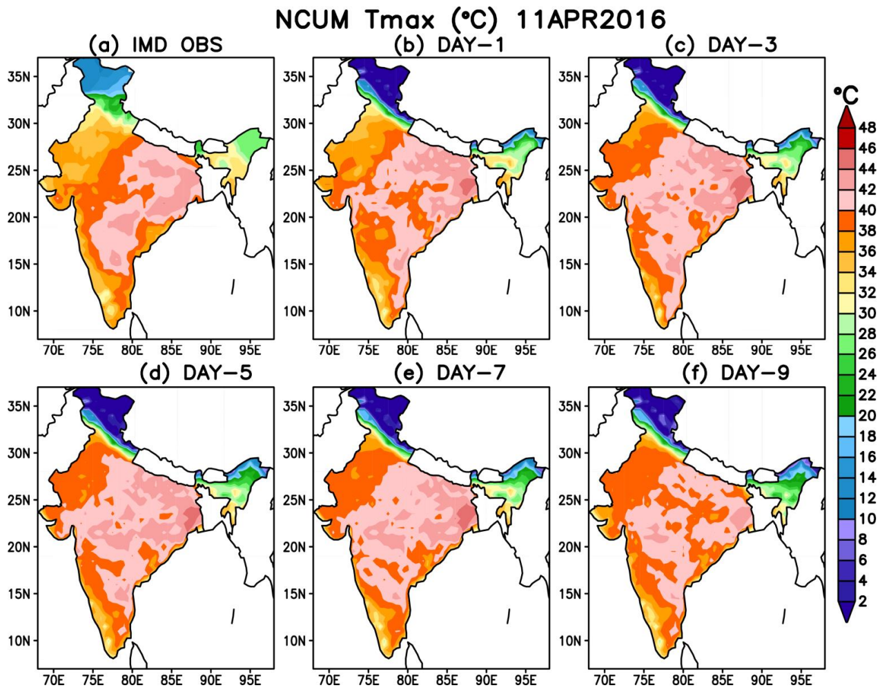
Figure 5. Spatial distributions of Observed T_{max} and NCUM forecast T_{max} prevailing heat waves over, MP, Odisha, AP, 5 Telangana and some parts of Maharashtra on 11 th April 2016. (NCUM stand for NCMRWF Unified Model). [Observed data from India Meteorological Department and forecast data from NCMRWF]
