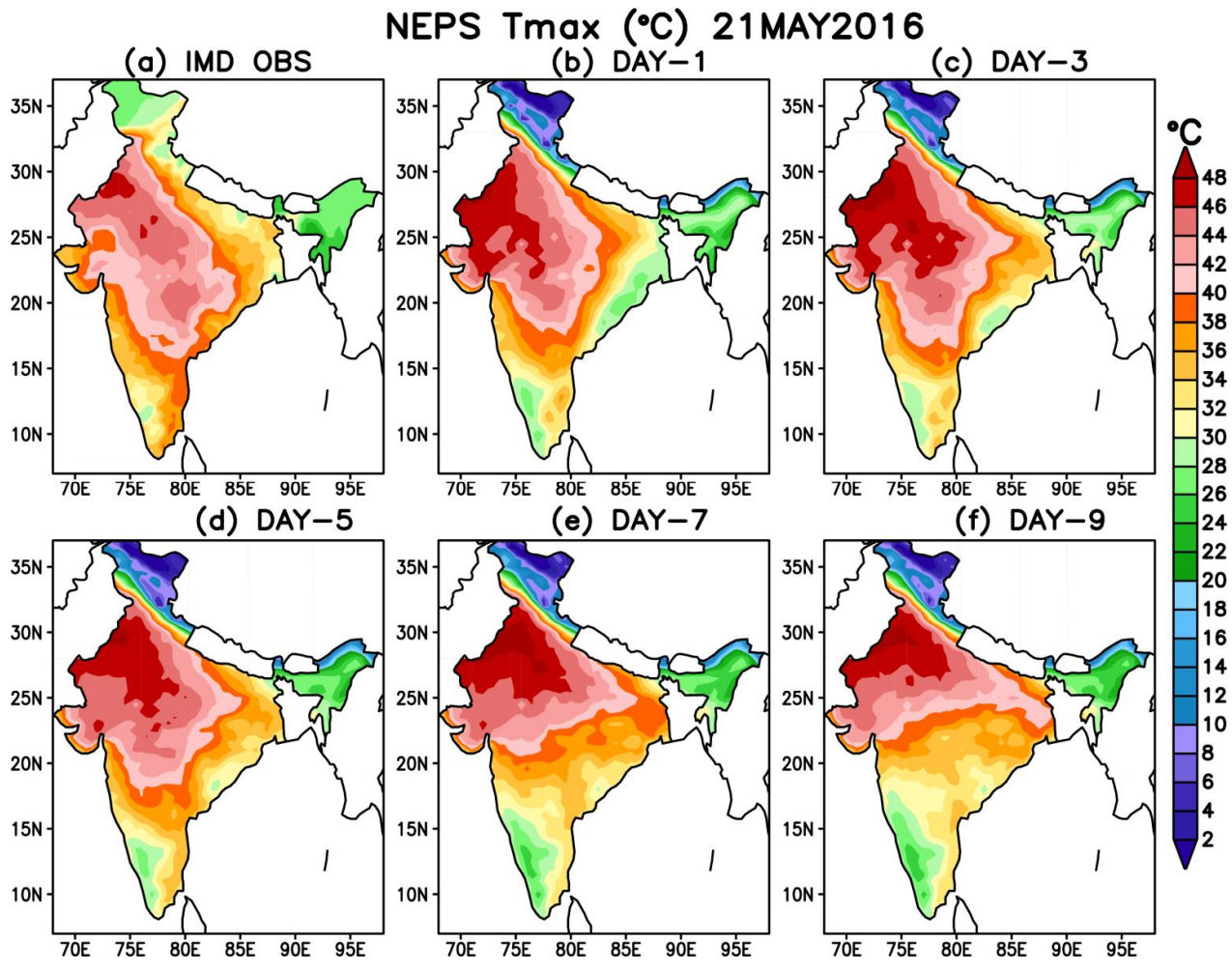
Figure 8. Spatial distributions of Observed T_{max} and NEPS forecast T_{max} prevailing heat waves over Rajasthan, MP, UP, Delhi, Haryana, Punjab and some parts of Maharashtra on 21 st May 2016. (NEPS stands for NCMRWF Ensemble Prediction System). [Observed data from India Meteorological Department and forecast data from NCMRWF]
