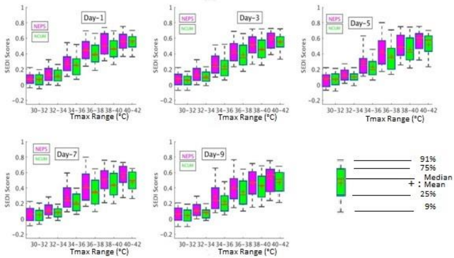
Figure 13. Box plots for Symmetric Extremal Dependence Index (SEDI) for NCUM and NEPS from March to May 2016. (NCUM stand for NCMRWF Unified Model and NEPS stands for NCMRWF Ensemble Prediction System)
