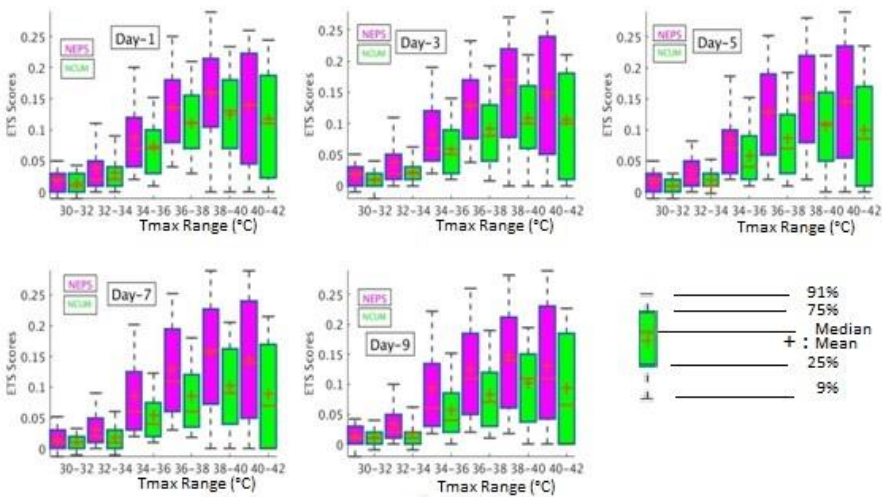
Figure 10. Box plots for Equitable Threat Score (ETS) for NCUM and NEPS from March to May 2016. (NCUM stand for NCMRWF Unified Model and NEPS stands for NCMRWF Ensemble Prediction System)
