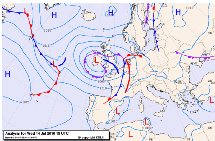
Figure 9. Weather chart of July 14, 1800 UTC. The chart shows the low pressure system south of Ireland and the cold front, displacing the warm continental air with cooler air from the Bay of Biscay, as the blue line with closed triangles.
