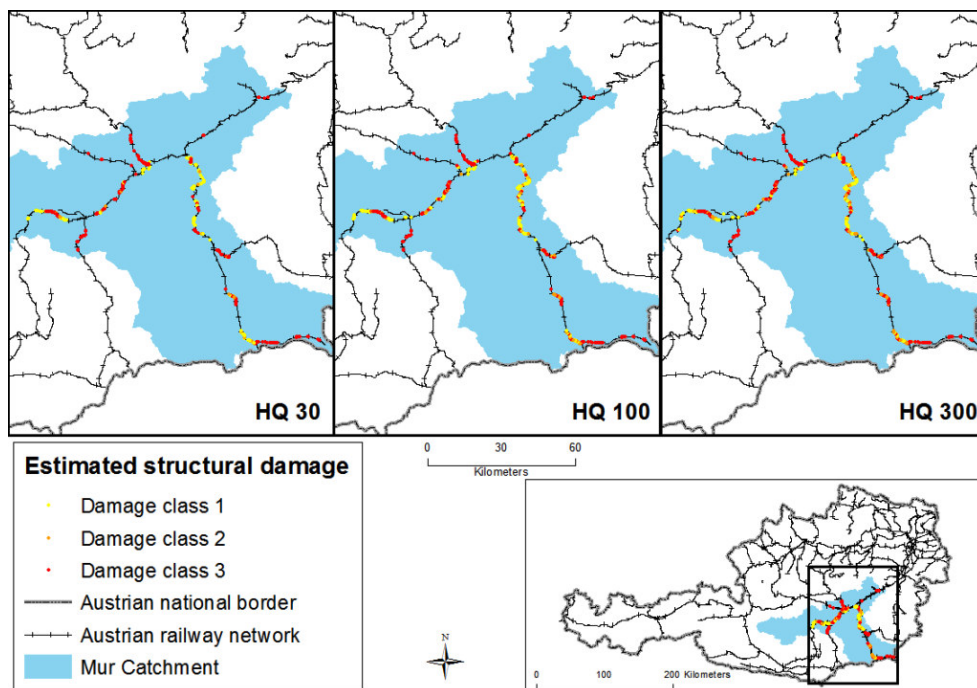
Figure 3. Estimation of damage potentials of the Austrian railway network within the Mur catchment. The left map shows the RAIL model results for a synthetic 30-year flood event. The results for a synthetic 100-year event are illustrated in the middle map. The right map covers the results of the model application using a 300-year design event as input.
