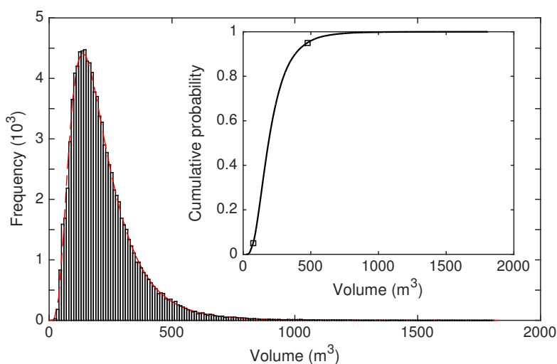
Figure 6. Histogram of the volumes having 1000 years return period fitted by a lognormal law (red dashed line). The empirical distribution function is plot in the box: the squares bound the 90% confidence interval.
