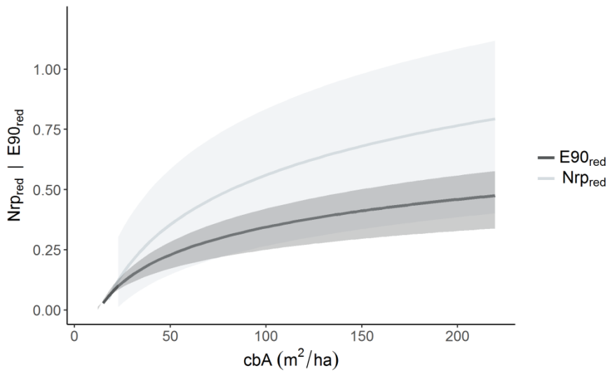
Fig. 6: Nrp red (light grey) and E90 red (dark grey) based on the simulation of all forest and terrain scenarios on the concave slope and depending on cbA using a logarithmic smoothing function and the respective 10% - and 90%-quantiles (shaded).
