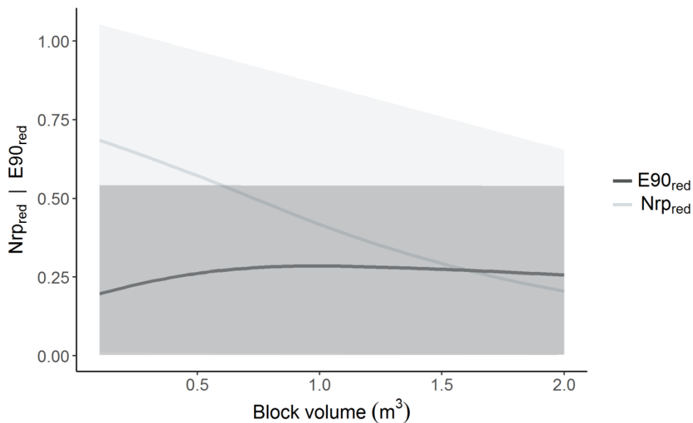
Fig. 7: Nrp red (light grey) and E90 red (dark grey) based on the simulation of all forest and terrain scenarios on a concave slope and depending on rock volume using a “loess” smoothing function and the respective 10% - and 90%-quantiles (shaded).
