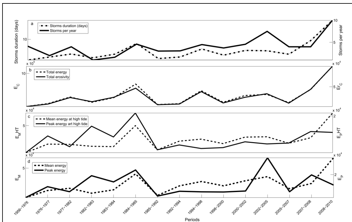
Figure 4. Cumulative energy ( E_C ) and wave erosivity ( E_{r_C} ), mean energy ( E_M ) and energy at high tide ( E_{M,ht} ), peak energy ( E_P ) and energy at high tide ( E_{P,ht} ) and storm duration for the periods between sets of photographs.
