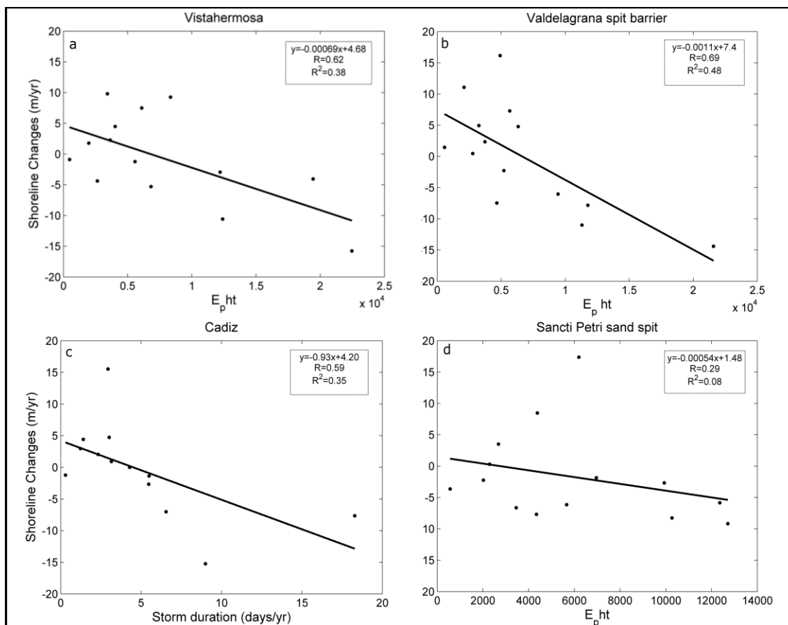
Figure 7. Examples of scatter plots of the correlation analysis for the study sites. Peak energy at high tide ( E_p ht) is shown for Vistahermosa, Valdelagrana and Sancti Petri units, while storm duration is shown for Cadiz unit.
