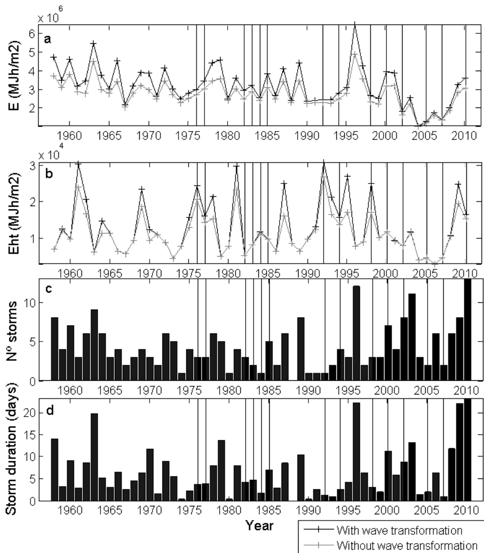
Figure 3. Temporal evolution of energetic parameters during the studied period: energy (E), energy at high tide (Eht), number of storms and storm duration. The dates of the available photographs are shown with vertical lines. The effect of wave transformation in E and Eht is shown for Cadiz site.
