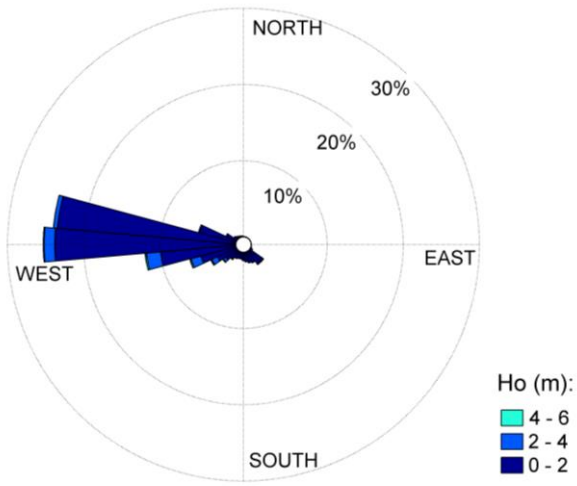
Figure 2. Wave height record from 1956 to 2010 in Cadiz buoy.
