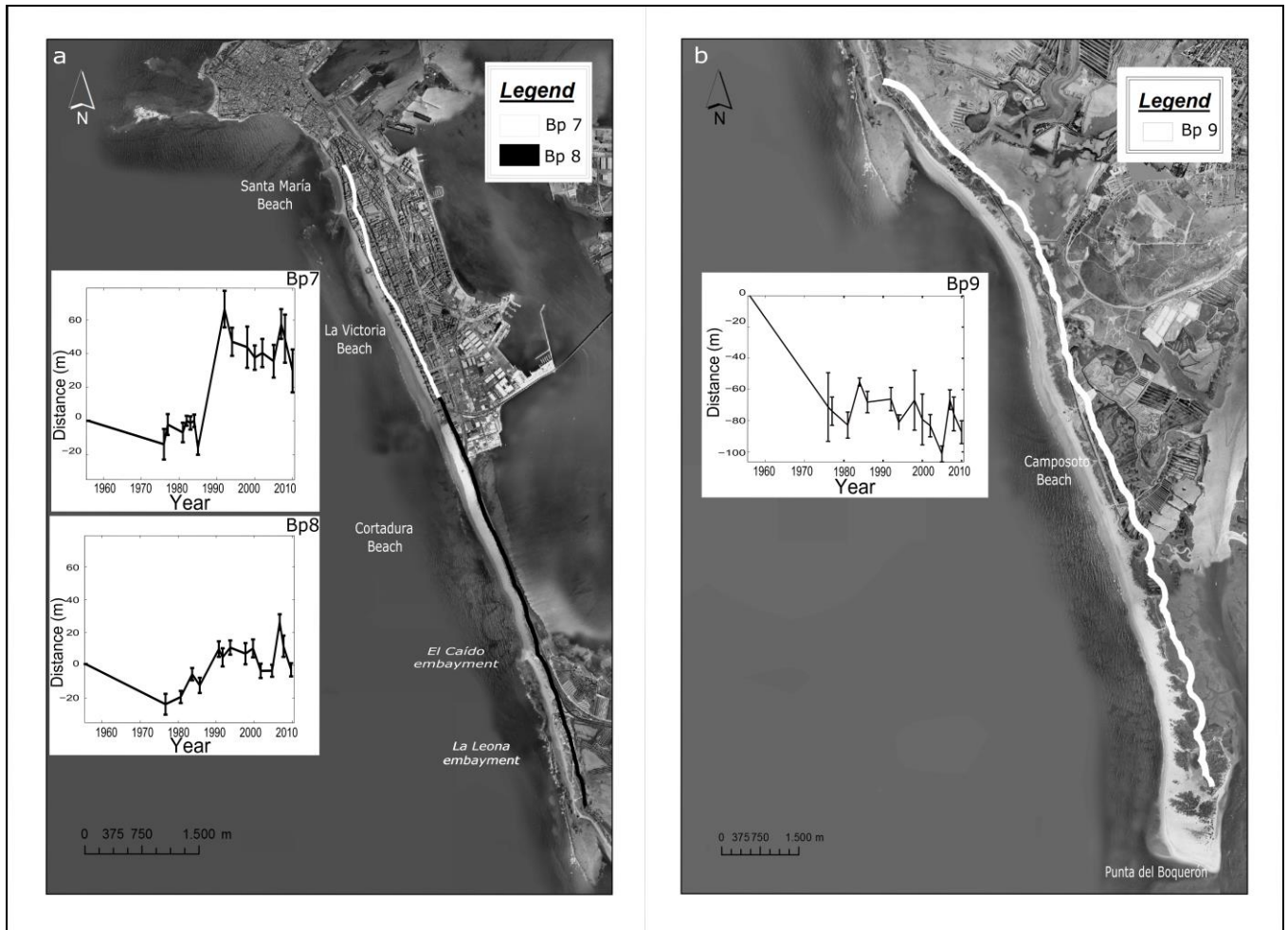
Figure 6. Shoreline trends of Cadiz (a) and Sancti Petri (b) sites classified by behavioural patterns (BP). Error bars represent alongshore variability.
