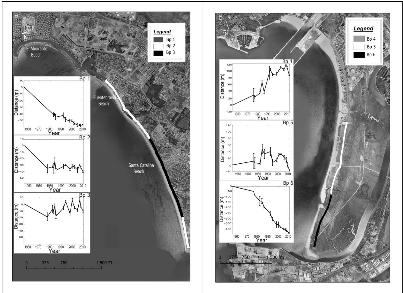
5 Figure 5. Shoreline trends of Vistahermosa (a) and Valdelagrana (b) sites classified by behavioural patterns (BP). Error bars represent alongshore variability.
