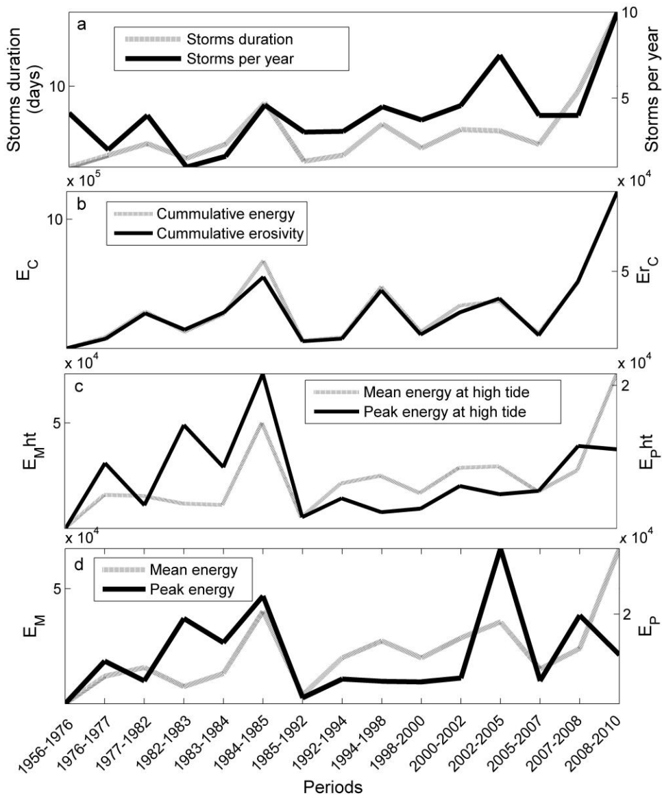
Figure 4. Cumulative energy ( E_C ) and wave erosivity ( Er_C ), mean energy ( E_M ) and energy at high tide ( E_{Mht} ), peak energy ( E_P ) and energy at high tide ( E_{Pht} ) and storm duration and frequency for the periods between sets of photographs.
