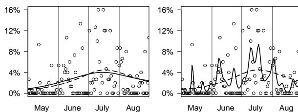
Figure 8. Local fits for the location E. Circles show empirical estimates. For comparison the estimate of the full occurrence model is added (dashed line). Left: Solid line is the GAM evaluated by cross-validation with day-wise blocks. Right: Solid line is the GAM evaluated by cross-validation without day-wise blocks.
