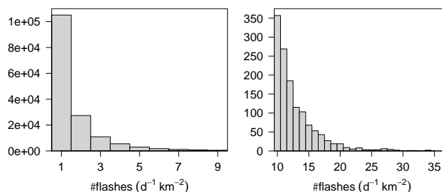
Figure 2. Daily frequency of 1 \text{ km} \times 1 \text{ km} grid cells in with counts of flashes (excluding zeros). The right panel shows a zoom into the tail of the distribution. The percentage of boxes with no flashes detected is 97.85%.
