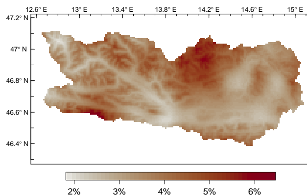
Figure 5. Climatological probability of lightning for July 20 in Carinthia on the 1 km x 1 km scale.
