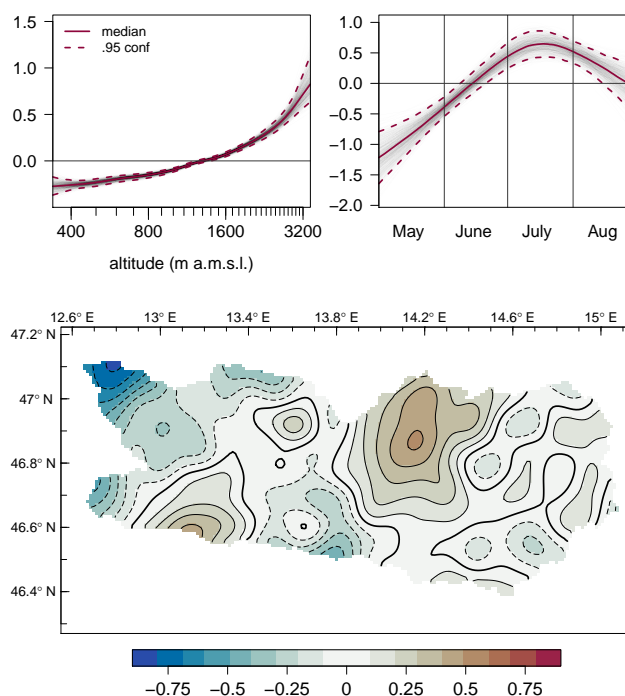
Figure 3. The effects of the occurrence model on the scale of the additive predictor. Top-Left: The altitude ( \log_{alt} ) effect. Ticks on the x-axis are set in 100 m intervals. The gray lines show 1000 estimates from day-wise block-bootstrapping. The solid red line is the median of the 1000 estimates, the dashed red lines are the 95% confidence intervals. Top-Right: The seasonal ( doy ) effect. Bottom: The spatial ( lon, lat ) effect. The plot shows the median of 1000 estimates from day-wise block-bootstrapping. The difference between two contour lines is 0.1. Dashed contour lines indicate negative values.
