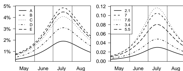
Figure 7. Seasonal climatologies for sample locations, which are highlighted in Figure 1. Left: Occurrence model. Right: Expected number of flashes. The legend shows expected number of flashes accumulated over the lightning season.
