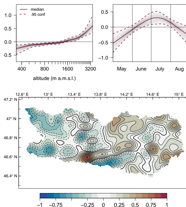
Figure 4. The effects of the intensity model on the scale of the additive predictor. Labeling is analog to Fig. 3. Top-Left: The altitude ( \log alt ) effect. Top-Right: The seasonal (day) effect. Bottom: The spatial ( \log lon, lat ) effect.
