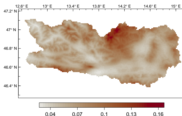
Figure 6. Expected (climatological) number of flashes for July 20 in Carinthia on the 1 \text{ km} \times 1 \text{ km} scale.
