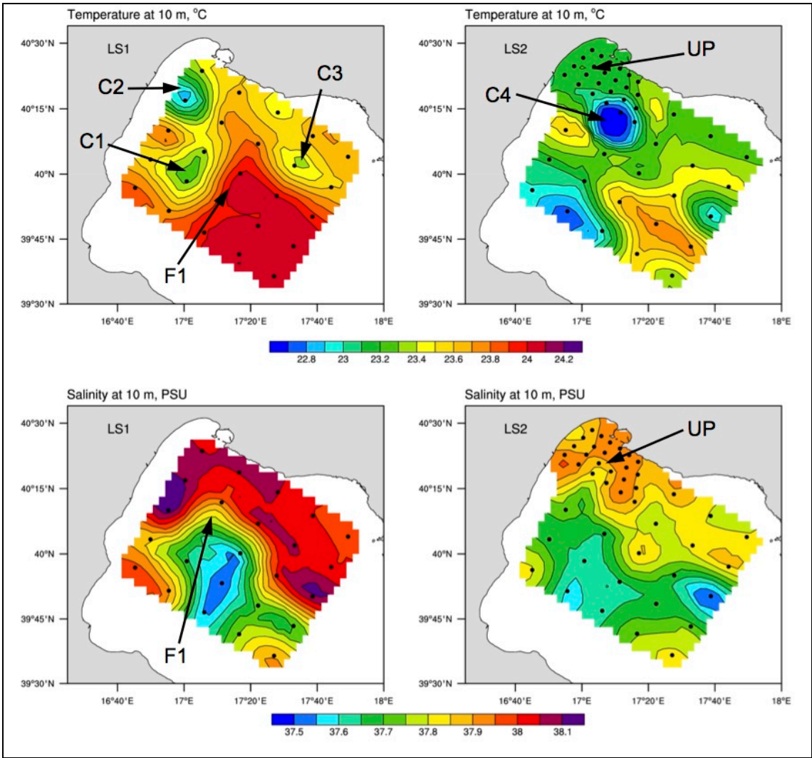
5 Fig. 10 Temperature and salinity objective mapping at 10 m. Left top and bottom panel: LS1 temperature and salinity fields. Right top and bottom panel: LS2 temperature and salinity fields. Symbols indicate four cold core eddies (C1, C2, C3, C4), the temperature and salinity front (F1) and the upwelling area (UP).
