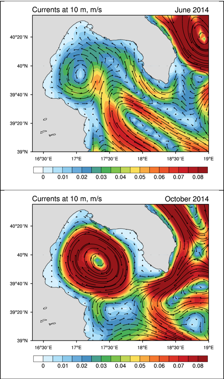
Fig. 2 Monthly mean surface currents from reanalysis (Pinardi et al., 2015) in the Gulf of Taranto. Top panel: June 2014. Bottom panel: October 2014. The units are \text{m s}^{-1} and the color indicates the amplitude
