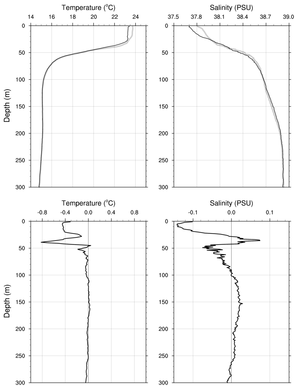
Fig. 6 Superimposed mean temperature and salinity LS1 and LS2 profiles and differences. Top left: LS1 (grey line) and LS2 (black line) mean temperature profiles. Top right: LS1 (grey line) and LS2 (black line) mean salinity profiles. Bottom left: LS2-LS1 mean temperature difference. Bottom right: LS2-LS1 mean salinity difference.
