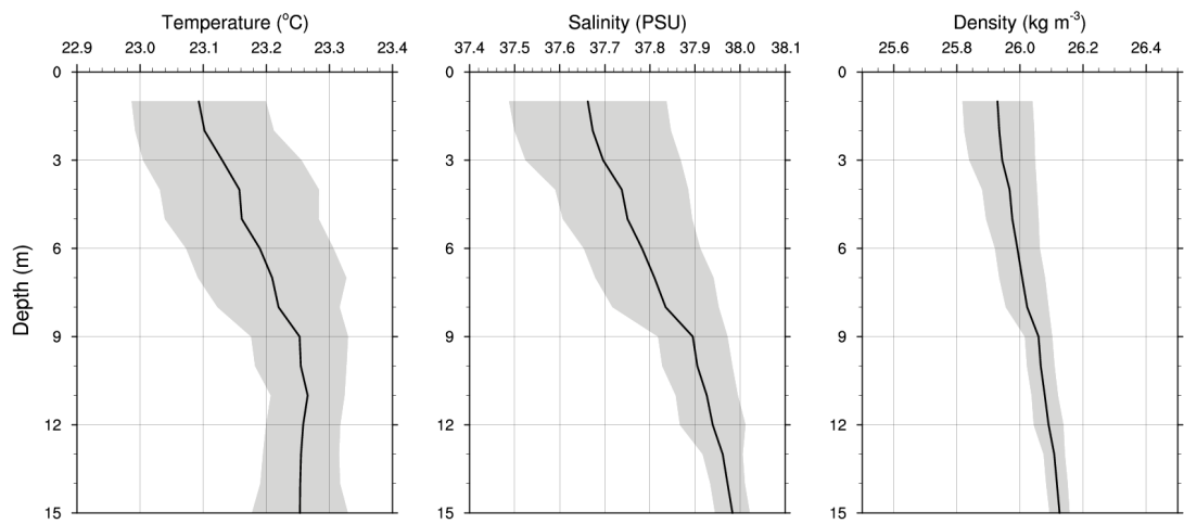
Fig. 9 Mar Grande horizontal average temperature (left), salinity (center) and density (right) profiles for October 5, 2014.
