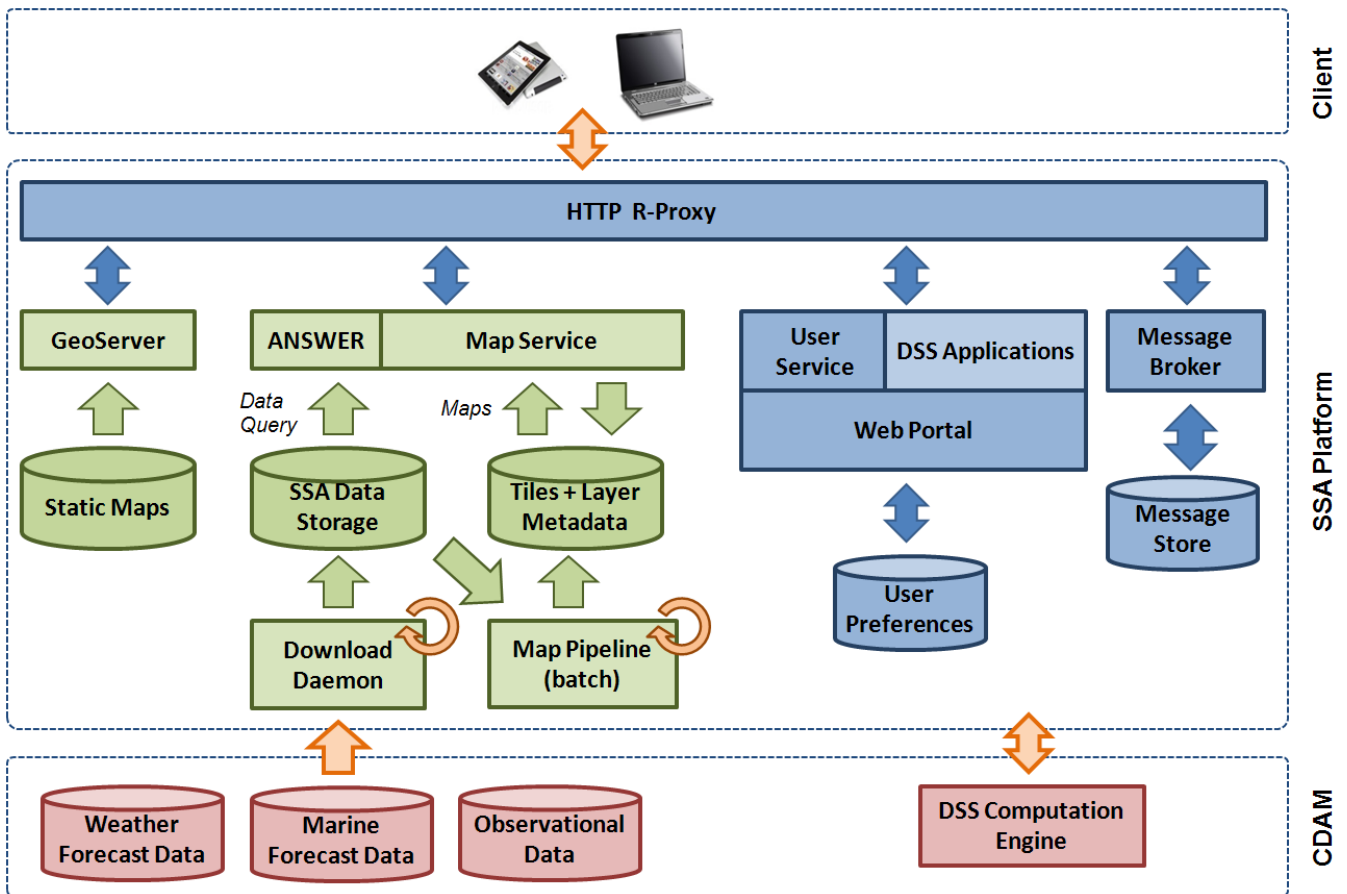
Figure 1. SSA Platform architecture (color key: blue for frontend components, green for map components, red for external modules or externally produced data)
