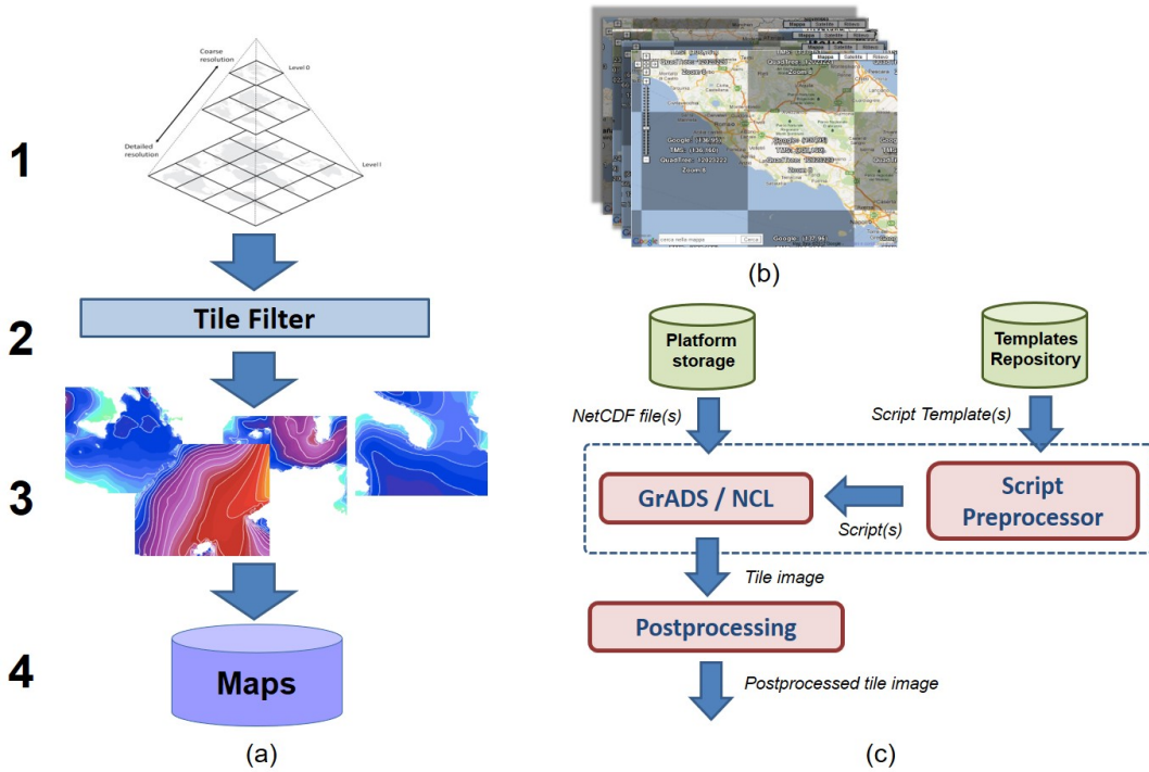
Figure 4 Tiled map generation
