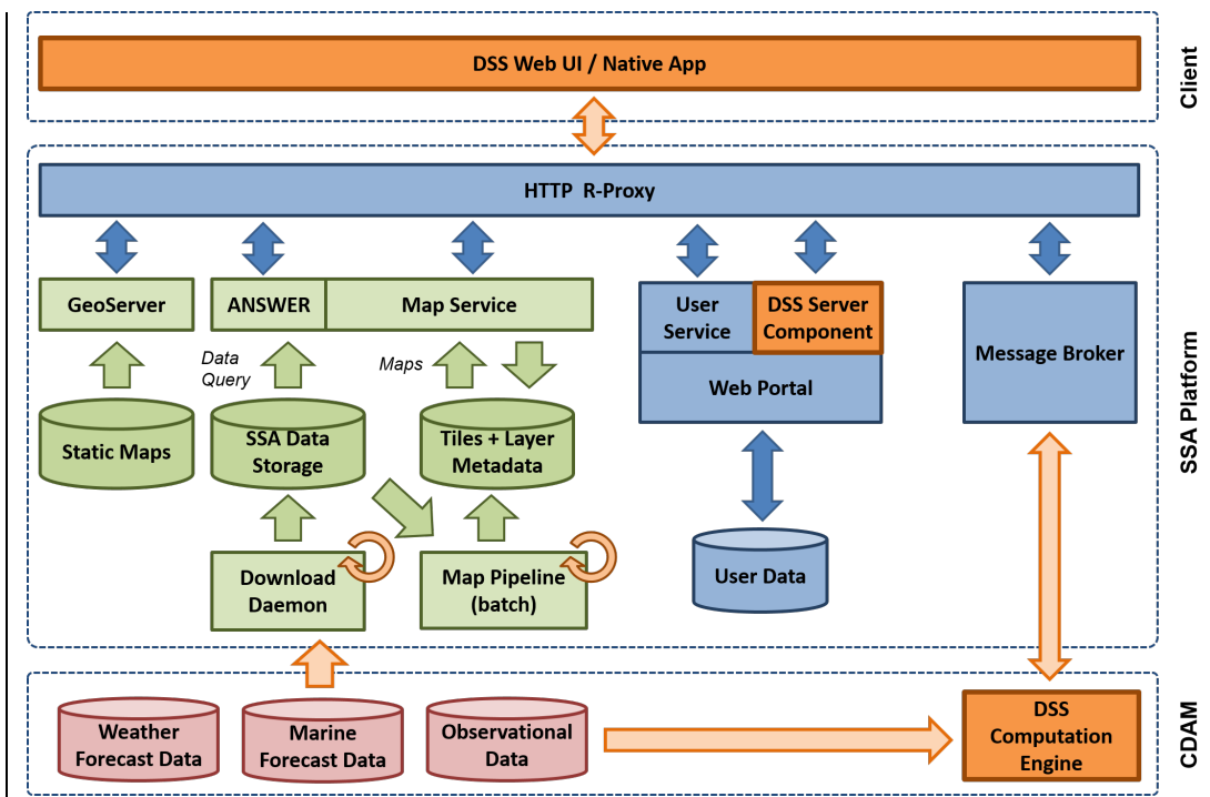
Figure 1 SSA Platform architecture (color key: blue for frontend components, green for map components, red for external modules or externally produced data, brown / orange for the DSS-specific components and interactions)
