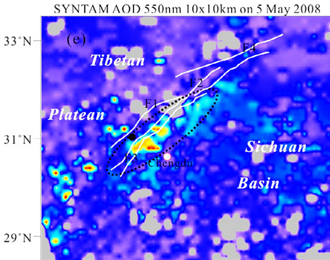
Fig. 1. Abnormal satellite-based AOD pattern one week before the 2008 Wenchuan EQ
