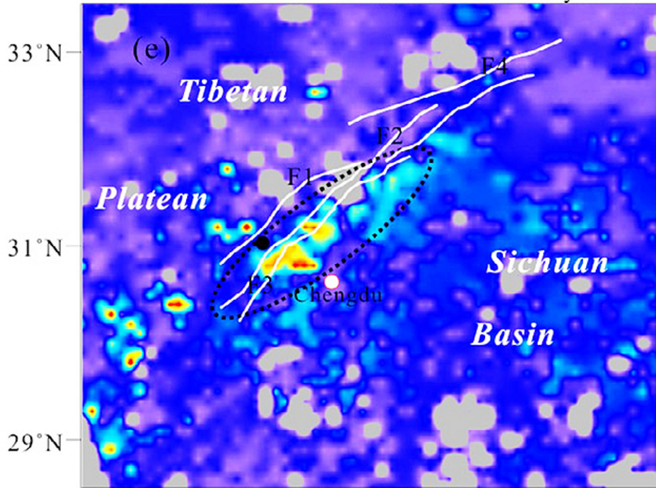
Fig. 1. Abnormal satellite-based AOD pattern one week before the 2008 Wenchuan EQ
