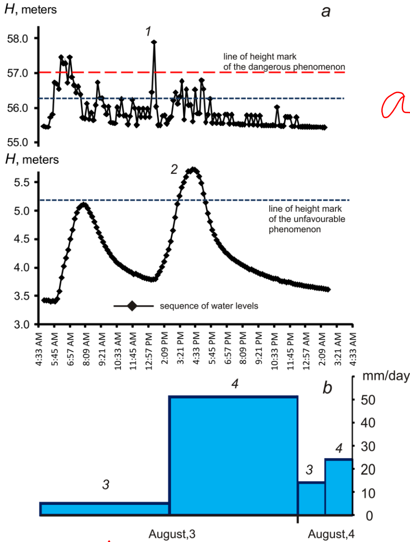
Figure 3. a) b) c) Graphs of fluctuations of water level of the Vulan River (a) and the diagram of the amount of daily rainfall (b) from August 3 - 4, 2013. Symbols: 1 – gauging station of Tekos (at 13 km upstream of the river mouth), 2 – gauging station of Arkhipo-Osipovka (in a river mouth); 3 – rainfall at meteorological station Gelendzhik, 4 – rainfall at meteorological station Dzhubga. Levels are relative to gauge-datum. The velocity of the flood was 2.4 km/s (at a longitudinal gradient on the reach of 0.004)
