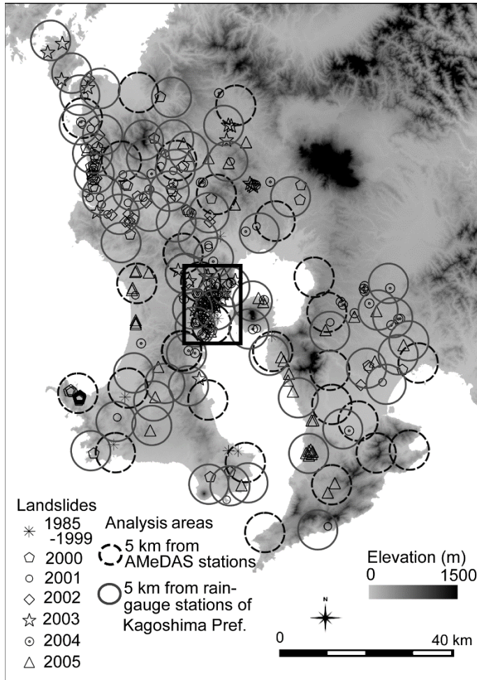
Figure 4. Locations of the Shirasu landslides in our database from 1985 to 2005 together with rain gauge stations in Kagoshima Prefecture. Rectangle shows the concentration of more than one-third of these damaging landslides in Kagoshima City.
