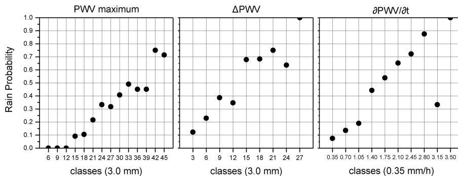
Figure 5. Probability of rain in the 2012 dataset as a function of PWV maximum (left panel), PWV maximum increase ( \Delta PWV, middle panel) and PWV rate of change ( \partial PWV/ \partial t , right panel). The x axis is represented by the top upper interval limit of the class, where the interval is 3.0, 3.0 mm and 0.35 \text{ mm h}^{-1} respectively.
