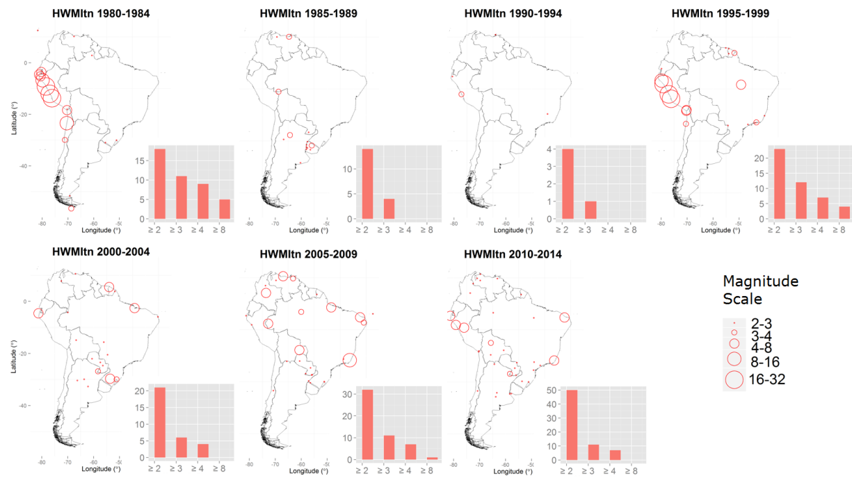
Figure S1 Magnitude of Heat Wave Index of minimum temperature (HWMI tn ) for 5-year periods from 1980 to 2014.
