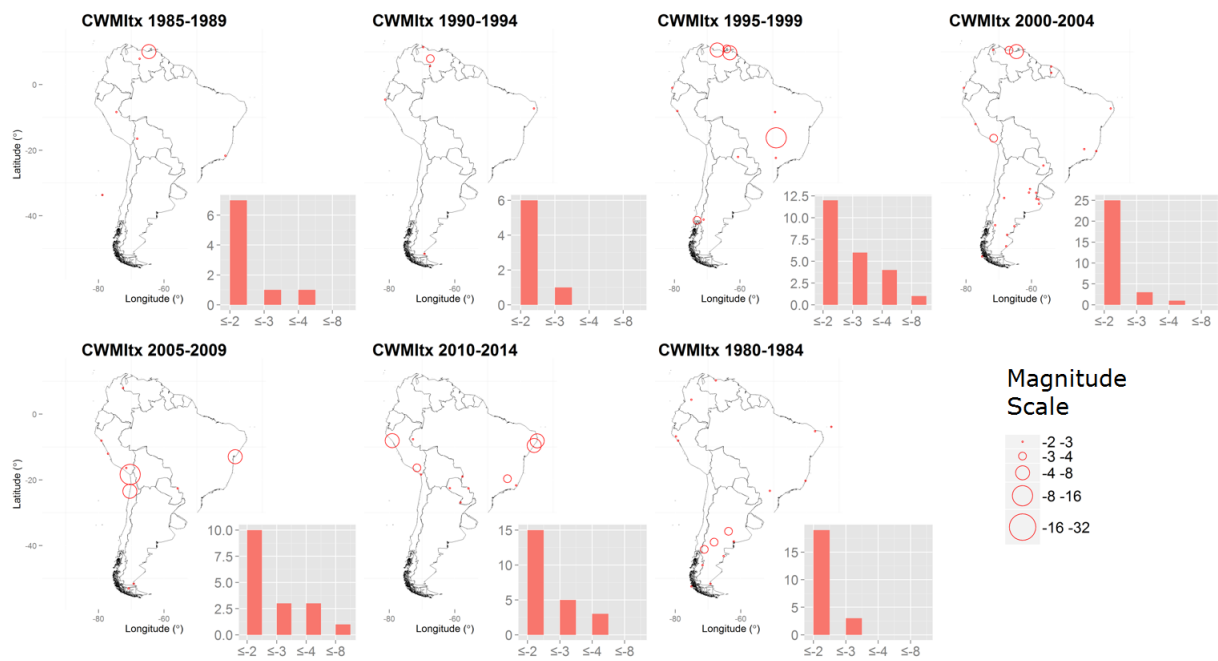
Figure S2 Magnitude of Cold Wave Index of maximum temperature ( CWMI_{tx} ) for 5-year periods from 1980 to 2014
