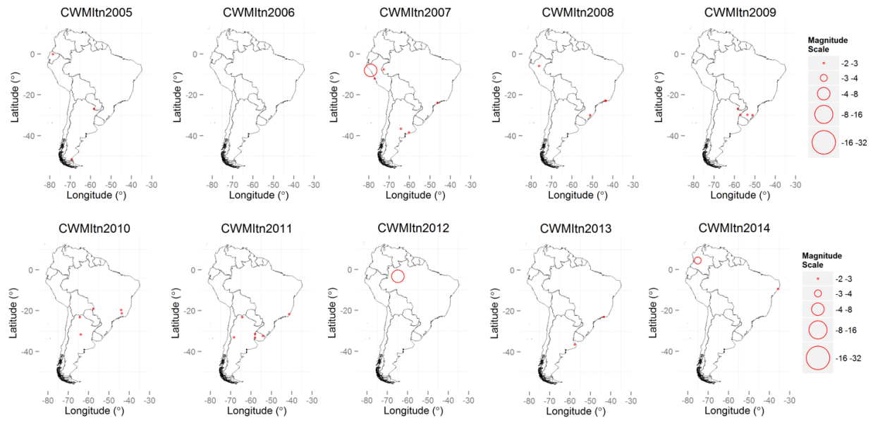
Figure S4 Annual values of Magnitude of Cold Wave Index of minimum temperature (CWMI tn ) from 1980 to 2014.
