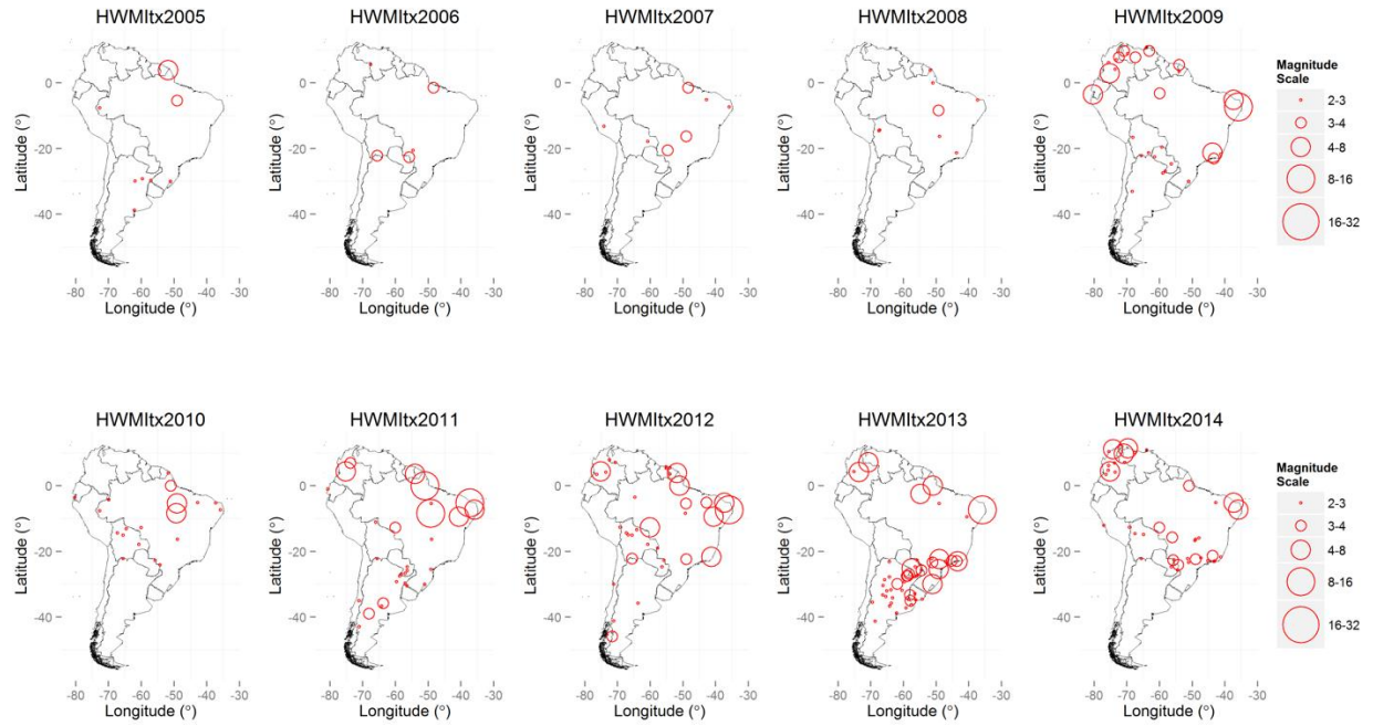
Figure S3 Annual values of Magnitude of Heat Wave Index of maximum temperature (HWMI tx ) from 1980 to 2014.
