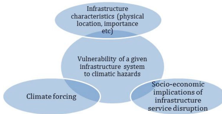
Figure 3. Vulnerability model.
