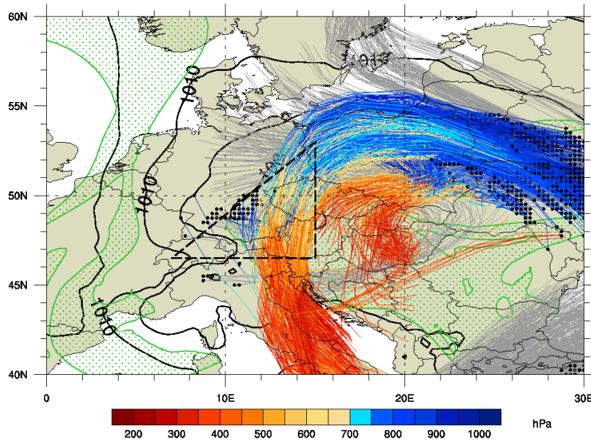
Fig. 1. As Figure 6b BUT with a weaker ascent criterion of 500hPa (48h) \hat{-1} , and trajectories plotted only with six-hourly position output.
