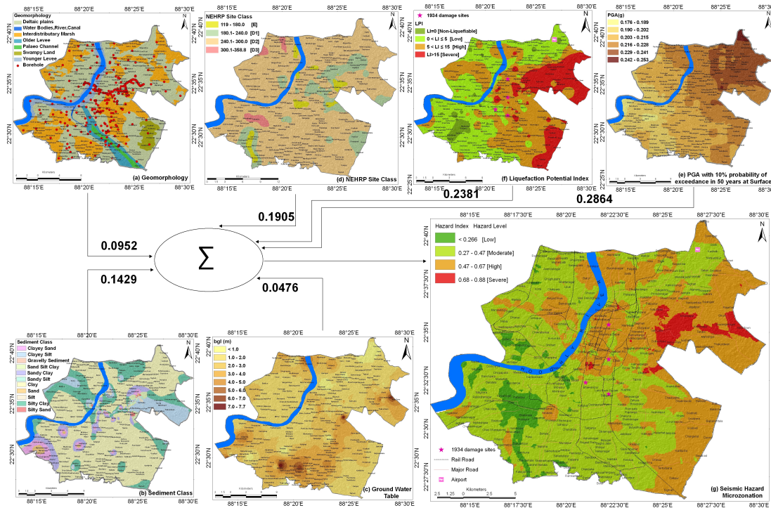
Fig. 7. Fig. 13. Seismic Hazard Microzonation for Kolkata showing the weights assigned to each theme labeled according to hazard contribution, (a) Geomorphology (b) Sediment Class, (c) Ground Water T
