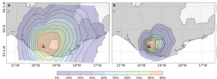
Fig. 10. Probability maps (%) for ground accumulation associated with a long-lasting 2010-type eruption of Eyjafjallajökull volcano. (a) LLOE, threshold of 1 kg m -2 ; (b) LLOES, threshold of 10 kg m -2 . Eruption parameters are summarized in Table 3 and Fig. 6.
