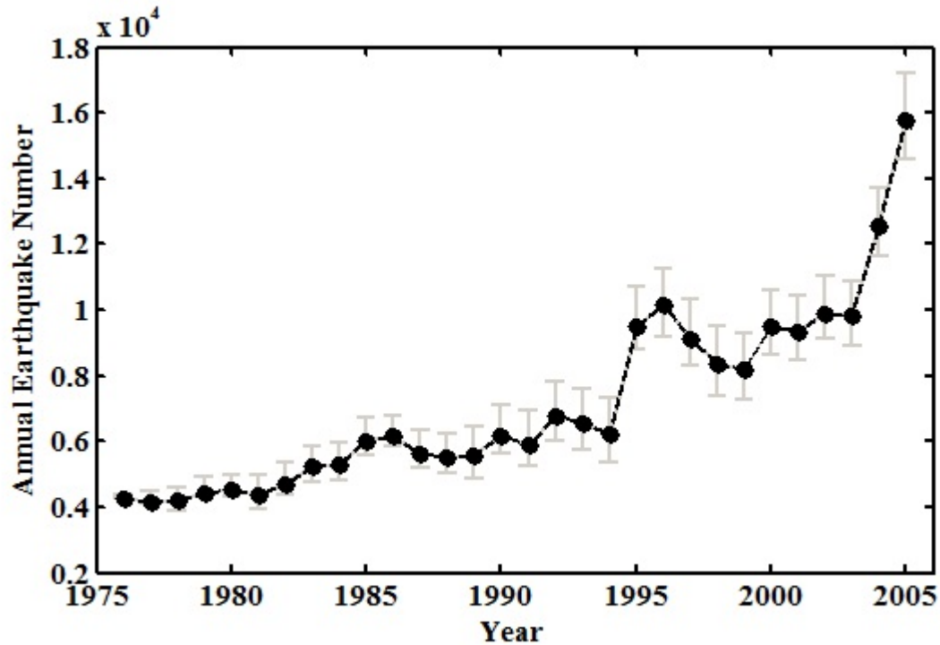
Fig. 1. Bootstrap confidence bounds of standard deviation of the global earthquake rate data using 1000 bootstrap samples.
