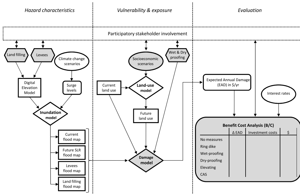
Fig. 1. Overview of methods applied in this paper (Filled shape indicate use of participatory developed information, ovals are external scenarios, diamonds are models, squared boxes are maps, polygons are adaptation strategies, and rounded squared boxes are evaluation criteria).
