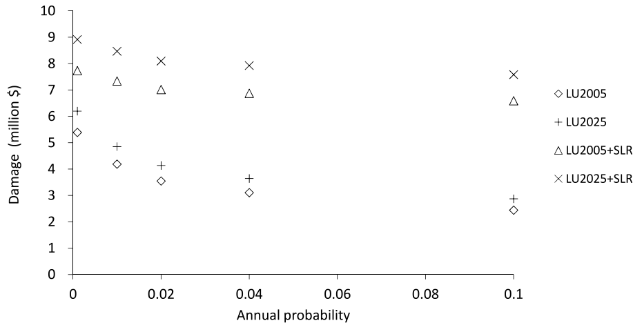
Fig. 7. Annual probability and damage curves for different combinations of land-use and sea-level scenarios.
