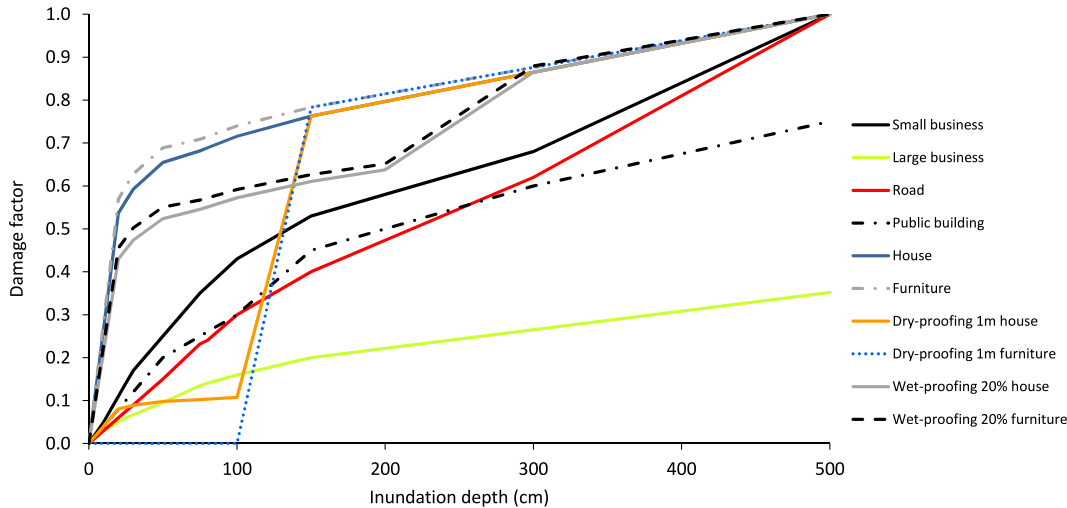
Fig. 3. Stage-damage curves as used in this study, including examples of dry and wet-proofing.
