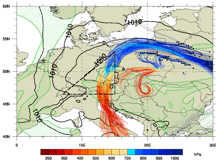
Fig. 2. Original Figure 6b with ascent criterion 600hPa (48h) \{ \} \{ -1 \} \{ \} , and trajectories plotted with one-hourly position output.
